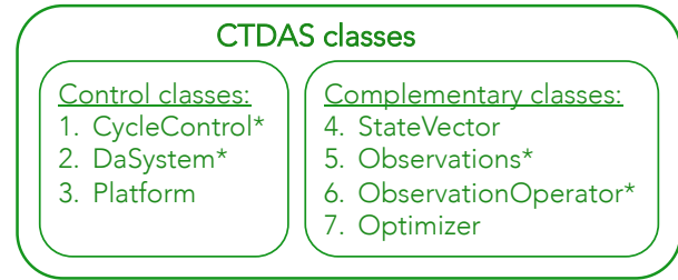
Figure 1. Overview of the 7 Python classes that comprise the CTDAS code base. Asterisks indicate passing information to the code through external run-control files.
