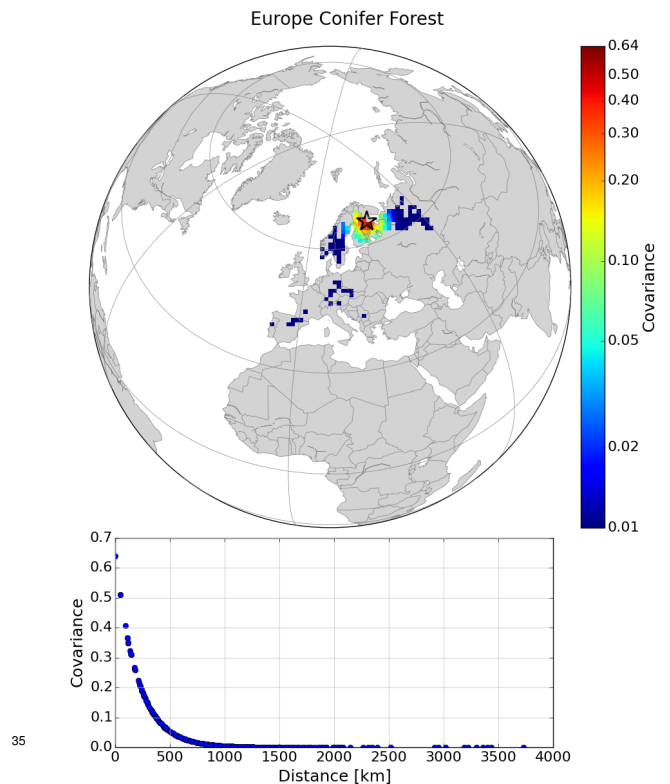
Figure 2. Error correlation in the gridded state vector setup for a specific grid box (indicated by the black star) in the European Conifer Forest region (with length scale 200 km) with the other grid boxes in that region (top panel) and versus distance (bottom panel).
