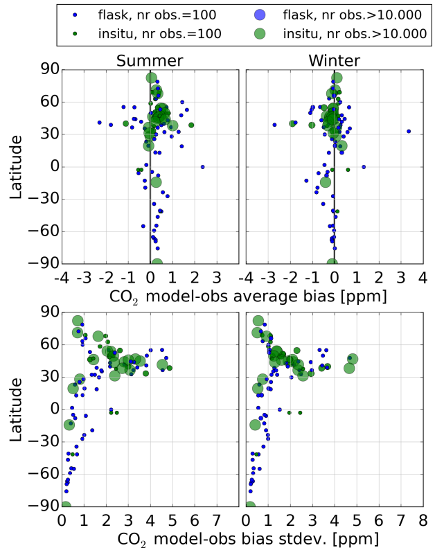
Figure 6. Latitudinal distribution of the average posterior residuals (top) and their standard deviations (bottom) per site over the period 2001-2015, for Northern Hemisphere summer (left) and winter (right). The residuals are calculated as the difference of the simulated minus observed \text{CO}_2 mole fractions for all assimilated observations. Assimilated values do not include \text{CO}_2 mole fractions of which their observed–forecasted value exceeds three times the prescribed model-data mismatch.
