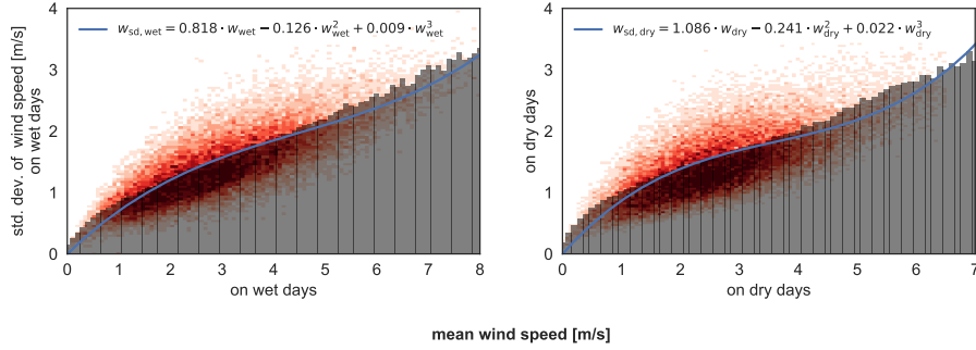
Figure 11. Correlation of standard deviation of wind speed on wet and dry days to the corresponding monthly mean. The y-axes show the standard deviation, the x-axes the mean on wet or dry days respectively. The blue line corresponds to the best fit line, a third order polynomial to the underlying red density plot. The black bars have a width of 0.1 \text{ m s}^{-1} , the accuracy of the input data, and indicate the mean standard deviations for the given interval range. Parameters of the fits are also shown in table 1.
