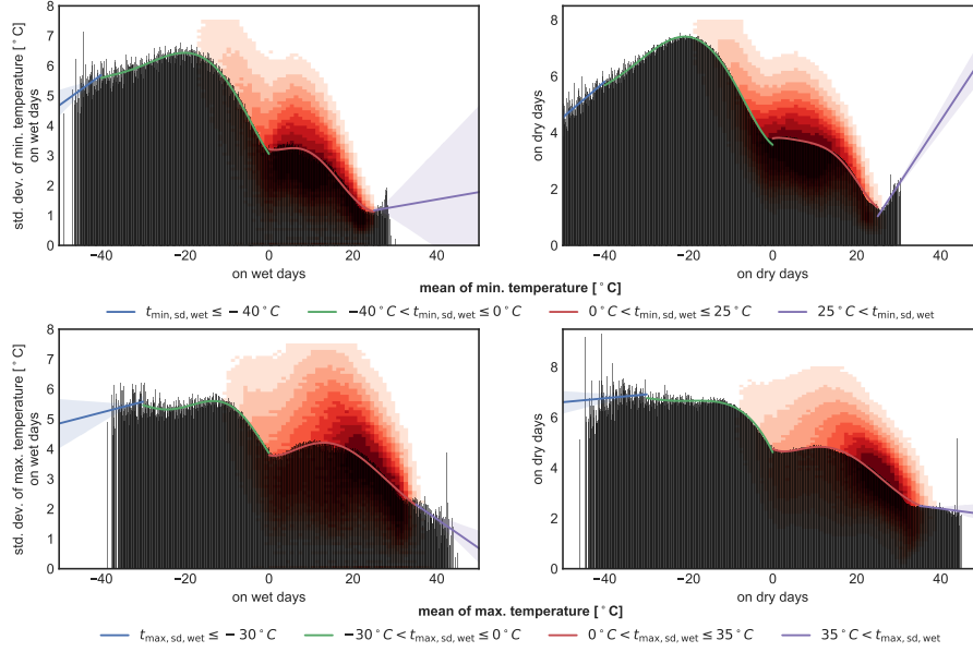
Figure 7. Correlation of standard deviation of the minimum and maximum temperature on wet and dry days to the monthly mean. The y-axes show the standard deviation, the x-axes the mean on wet or dry days respectively. The bars have a width of 0.1^{\circ}\text{C} (the data accuracy) and indicate the mean standard deviation for a given mean minimum temperature in one month. The lines are fitted to these bars, where the green and red polynomials of order 5 are the use all the data below or above 0^{\circ}\text{C} respectively and the blue and violet lines are a linear extrapolation of the data below -40^{\circ}\text{C} (or -30^{\circ}\text{C} for T_{\text{max}} ) or above 25^{\circ}\text{C} (or 35^{\circ}\text{C} ) respectively. The red density plot in the background indicates the spread of the data. The bars and the density plot are based on the single month for each station (i.e. not the multi-year monthly series as for, e.g. mean temperature (figure 5 and 6)). Parameters of the fits are also shown in table 1.
