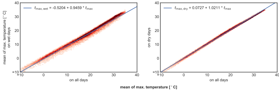
Figure 6. Correlation of maximum temperature on wet and dry days to the monthly mean. The y-axes show the mean maximum temperature on wet or dry days respectively, the blue line corresponds to the best fit line. Parameters of the fits are also shown in table 1.
