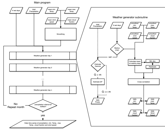
Figure 1. Schematic workflow of GWGEN. After smoothing the monthly input, the Markov Chain is used to decide, whether it is a dry or a wet day. If it is a wet day, we draw a random number from the Gamma-GP distribution. Furthermore, the other means of the variables ( \bar{T}_{\min/\max} , \bar{c} , \bar{w} ) are adjusted and their daily values are calculated using the estimated standard deviations and residuals. The wind speed furthermore undergoes a square root transformation before applying the cross correlation and in the end is corrected using the bias correction. A quality check in the end restricts our model to be within a 5% range of the observed total precipitation and to replicate the number of wet days from the input.
