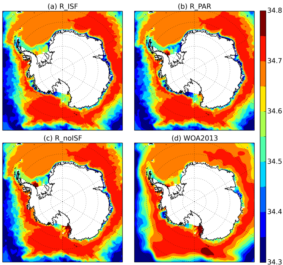
950 Figure 8: Salinity (PSU) averaged between 300 and 1000m (year 10, 1988) from a) R_ISF, b) R_PAR, c) R_noISF, d) World Ocean Atlas 2013 (Locarnini et al., 2013 and Zweng et al., 2013).
