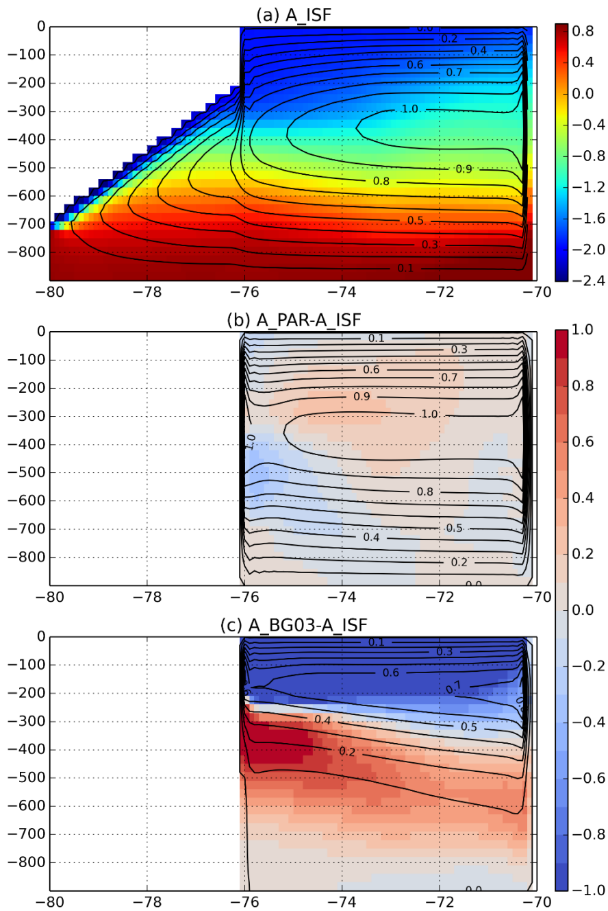
Figure 5: (a) Zonal mean temperature (°C) after 30 years of the run; in contour, the meridional overturning stream function (MOC) in the A_ISF experiment. b) Mean temperature difference (°C) with respect to A_ISF experiment (A_PAR-A_ISF); in contour, the MOC in the A_PAR experiment. c) as b) but for A_BG03.
