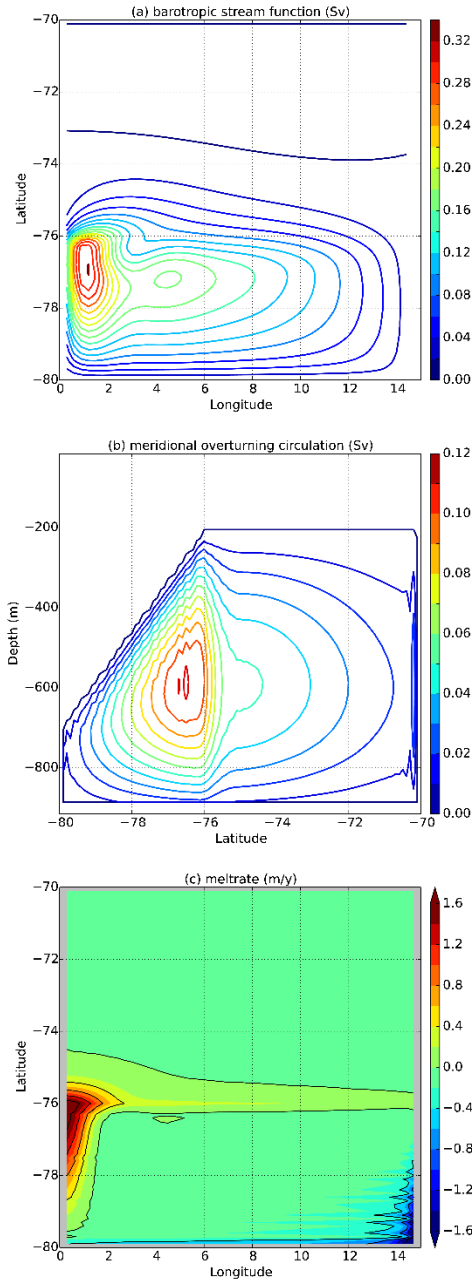
Figure 2: Near steady state (after 10000 days) solution of the I_30M ISOMIP experiment. a) Horizontal stream function ( \Psi ) in S_v with a contour interval of 0.02 S_v , b) Meridional overturning circulation (moc) in S_v with a contour interval of 0.01. c) Melt rate in m\ y^{-1} (negative for melting and positive for freezing) with a contour interval of 0.4 m\ y^{-1} .
