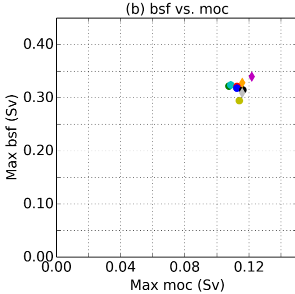
Figure 3: a) Total melting rate versus total freezing rate, and b) meridional overturning circulation versus barotropic stream function (bsf) for all the ISOMIP sensitivity experiments (I_5M, I_10M, I_30M, I_60M, I_100M, I_150M, I_31L, I_46L and I_75L). The simulations I_XXM are with constant vertical resolutions of XX m and a H_{\text{TBL}} of 30 m, the simulations I_XXMYYM are with constant vertical resolution of XX m and a H_{\text{TBL}} of YY m, Finally, the simulations I_XXL are with variable vertical resolution. Details are given in Table 2.
