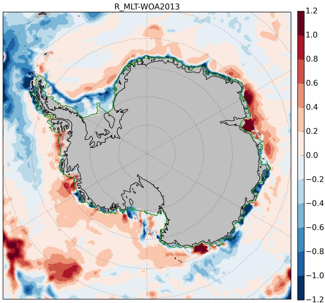
Figure 14: 300-1000m mean temperature differences between R_MLT (year 10, 1988) and observations from World Ocean Atlas 2013 (Locarnini et al., 2013 and Zweng et al., 2013). Grey area represents ice sheet, ice shelves or ocean shallower than 300m. The hatched area limited by the green line represents where the observational dataset is obtained by extrapolation.
