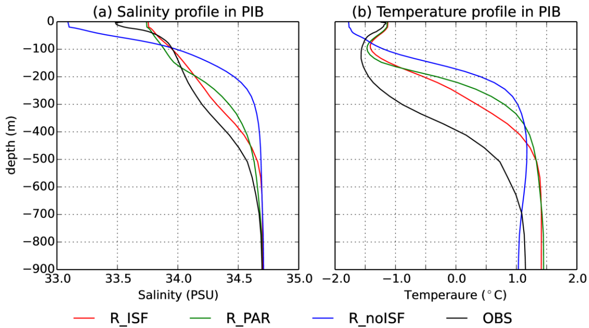
Figure 9: Profiles (year 10, 1988) in Pine Island Bay in R_noISF (blue), R_ISF (red) and R_PAR (green) of a) salinity and b) temperature. Climatology from 1994 to 2012 (Dutrieux et al, 2014) is in black.
