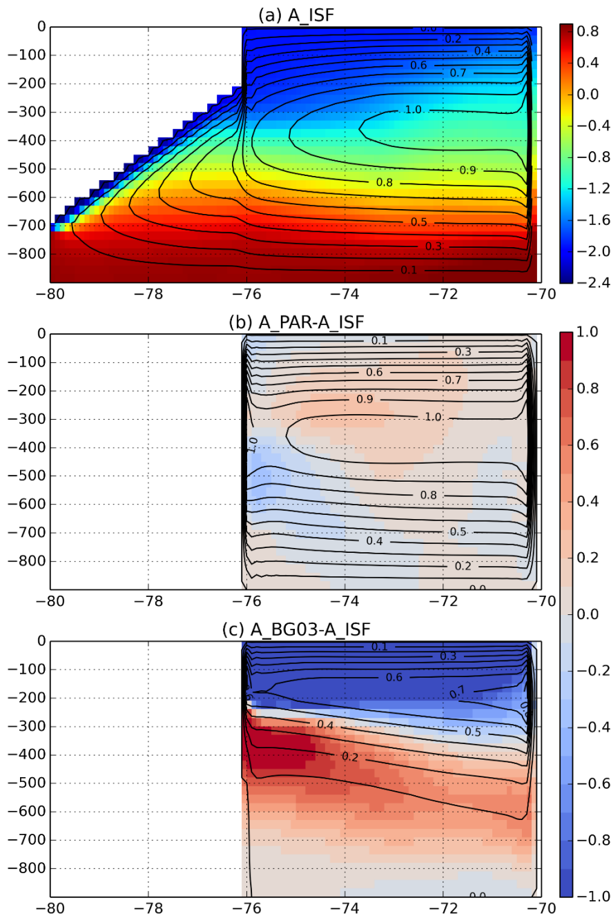
Figure 5: (a) Zonal mean temperature (°C) after 30 years of the run A_ISF ; in contour, the meridional overturning stream function (MOC) in the A_ISF experiment. b) Mean temperature difference (°C) with respect to A_ISF experiment (A_PAR-A_ISF); A_ISF ; in contour, the MOC in the A_PAR experiment. c) as b) but for A_BG03.
