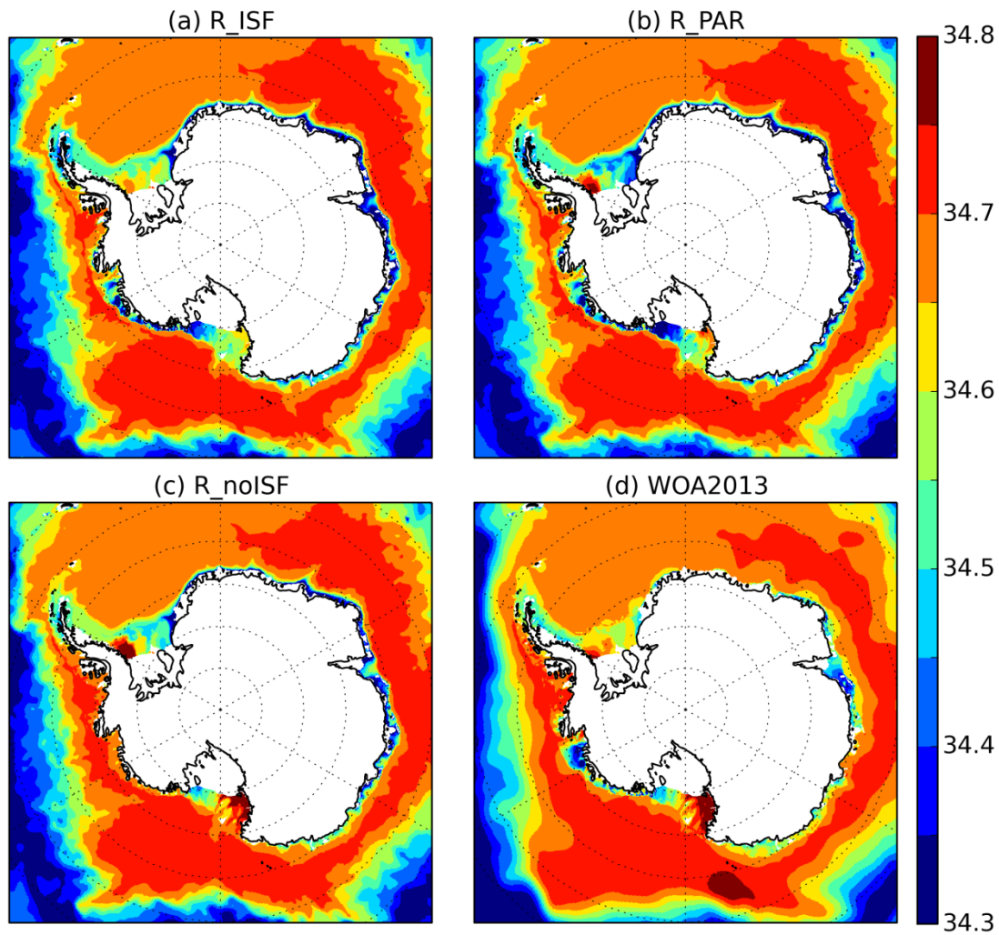
Figure 8: Salinity (PSU) averaged between 300 and 1000m ( year 10, 1988 ) from a) R_ISF, b) R_PAR, c) R_noISF, d) World Ocean Atlas 2013 (Locarnini et al., 2013 and Zweng et al., 2013).
