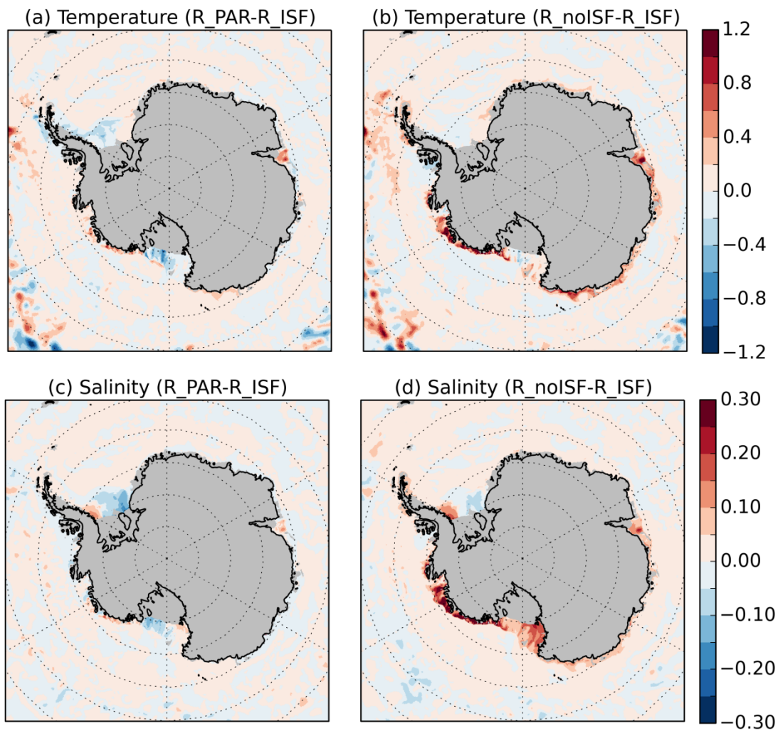
Figure 12: Map of temperature in ^{\circ}\text{C} (a,b) and salinity in PSU (c,d) differences between R_PAR and R_ISF (a,c) and R_noISF and R_ISF (b,d) averaged between 300 m and 1000 m.
