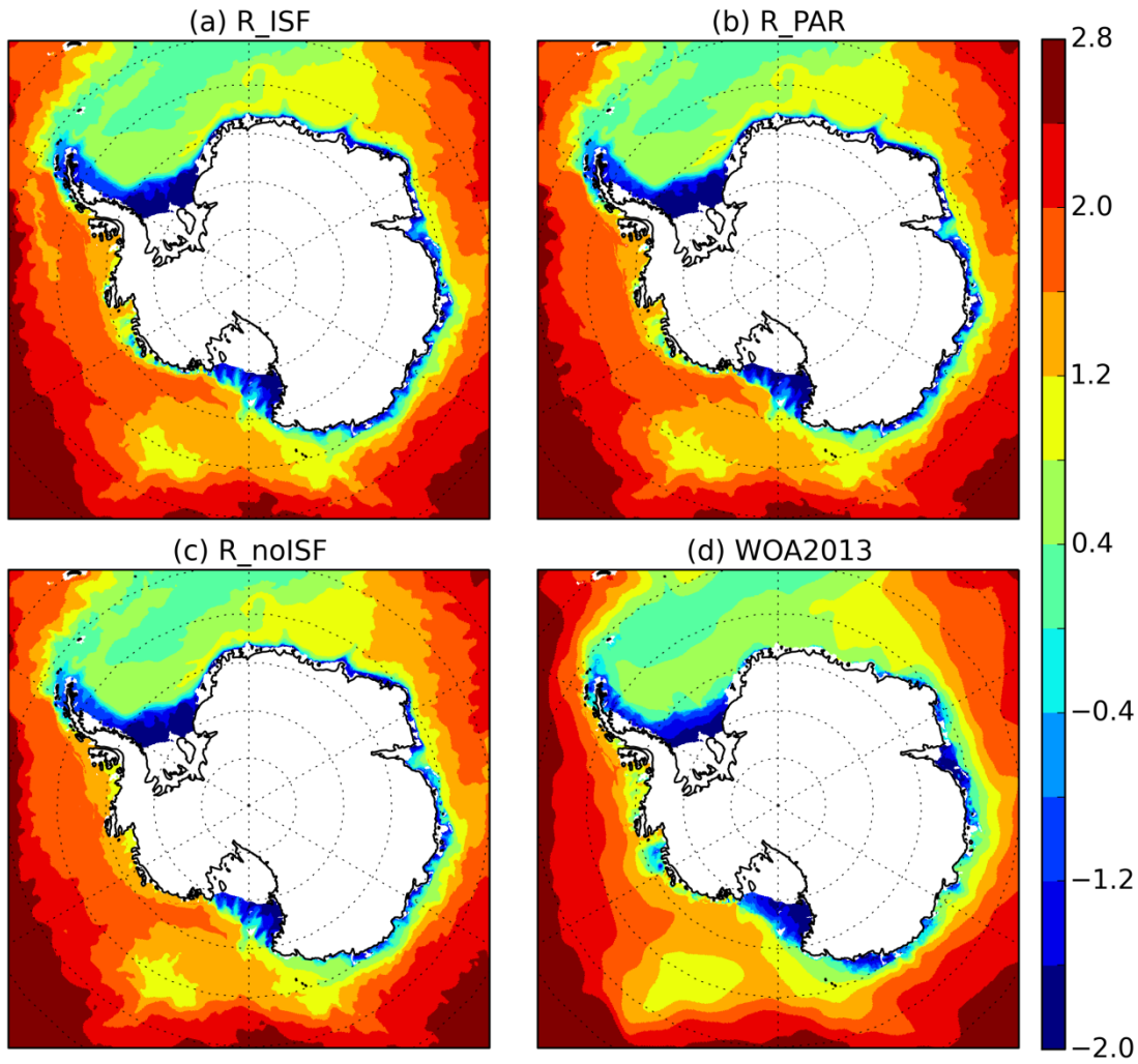
Figure 7: Temperature (°C) averaged between 300 and 1000m ( year 10, 1988 ) from a) R_ISF, b) R_PAR, c) R_noISF, d) World Ocean Atlas 2013 (Locarnini et al., 2013 and Zweng et al., 2013).
