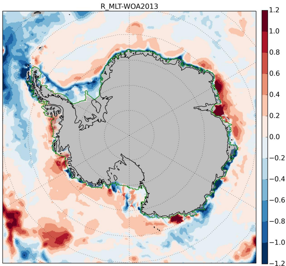
Figure 14: 300-1000m mean temperature differences between R_MLT ( year 10, 1988 ) and observations from World Ocean Atlas 2013 (Locarnini et al., 2013 and Zweng et al., 2013). Grey area represents ice sheet, ice shelves or ocean shallower than 300m. The hatched area limited by the green line represents where the observational dataset is obtained by extrapolation.
