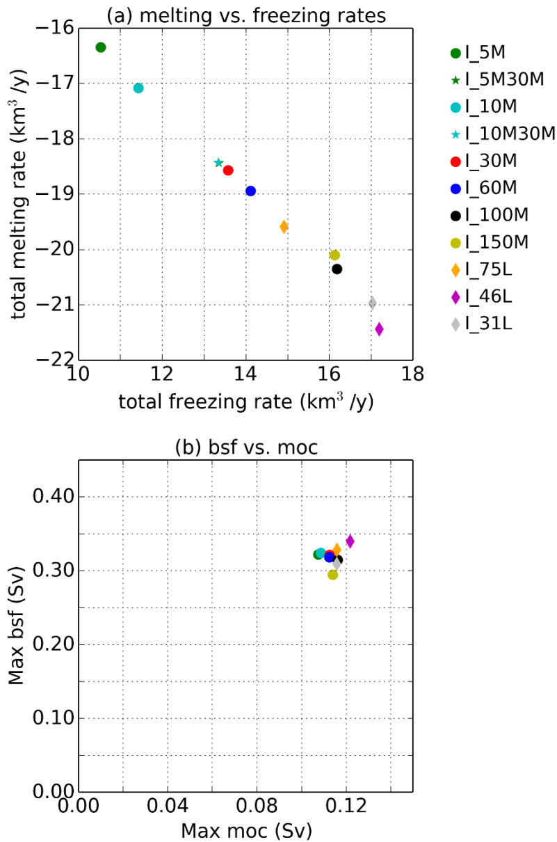
Figure 3: a) Total melting rate versus total freezing rate, and b) meridional overturning circulation versus barotropic stream function (bsf) for all the ISOMIP sensitivity experiments (I_5M, I_10M, I_30M, I_60M, I_100M, I_150M, I_31L, I_46L and I_75L). The simulations I_XXM are with constant vertical resolutions of XX m and a H_{TBL} of 30 m, the simulations I_XXMYYM are with constant vertical resolution of XX m and a H_{TBL} of YY m, Finally, the simulations I_XXL are with variable vertical resolution. Details are given in Table 2.
