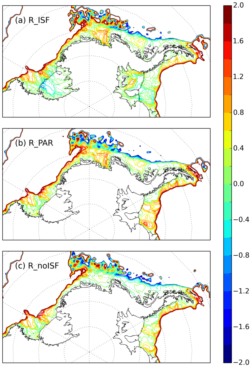
960 Figure 10: Barotropic stream function (Sv) on the Ross, Amundsen, Bellingshausen and Weddell continental shelves in a) R_ISF, b) R_PAR and c) R_noISF. Stream function isolines out of the \pm 2 Sv range are not plotted.
