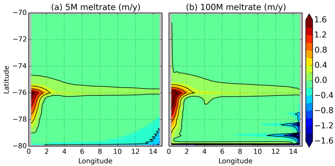
Figure 4: Melt rate in a) the 5M simulation, and b) the 100M simulation in \text{m y}^{-1} (negative for melting and positive for freezing) with a contour interval of 0.4 \text{ m y}^{-1} .
