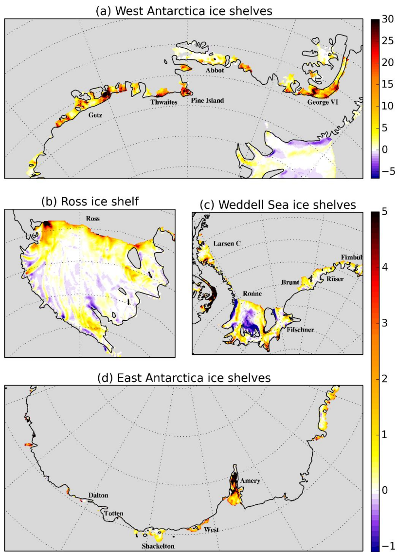
Figure 13: Ice shelf melting ( \text{m y}^{-1} , positive values mean melting) in the R_MLT simulation for a) the West Antarctic ice shelves, b) Ross Ice Shelf, c) Filchner-Ronne Ice Shelf and d) the East Antarctic ice shelves. Note that panels (a) and (b,c and d) have different colorbars.
