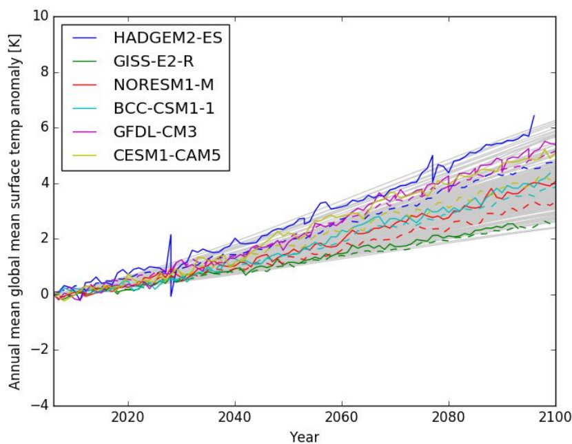
Figure 1: Annual mean global mean surface temperatures calculated from the CMIP5 AOGCM simulations under the RCP8.5 scenario (coloured solid lines). The annual mean global means from the HadAM3P (dashed lines) and MAGICC (grey lines) for RCP8.5 are also shown.
