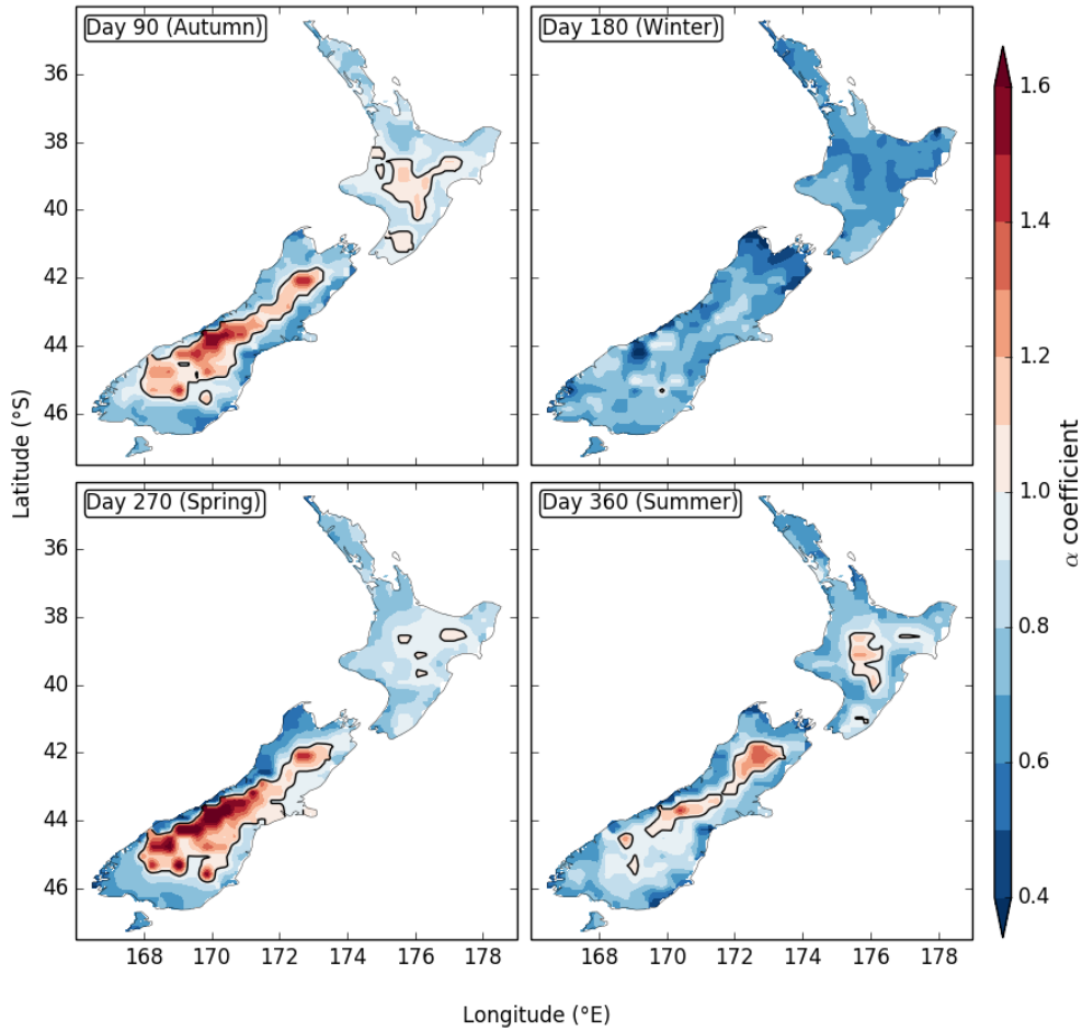
Figure 5. Maps of \alpha coefficients (unitless) which represent the sensitivity of changes in daily maximum surface temperature to changes in annual mean global mean maximum-surface temperature-temperatures for locations throughout New Zealand. The \alpha coefficients were derived from fits of Eq. (32) to daily time series of daily maximum temperatures at each grid point of the NorESM1-M RCM simulation. The annual mean global mean surface temperature anomalies were taken from the AOGCM-AGCM simulation that provided the boundary conditions for this particular RCM simulation. Black line-lines indicates \alpha values of 1.0.
