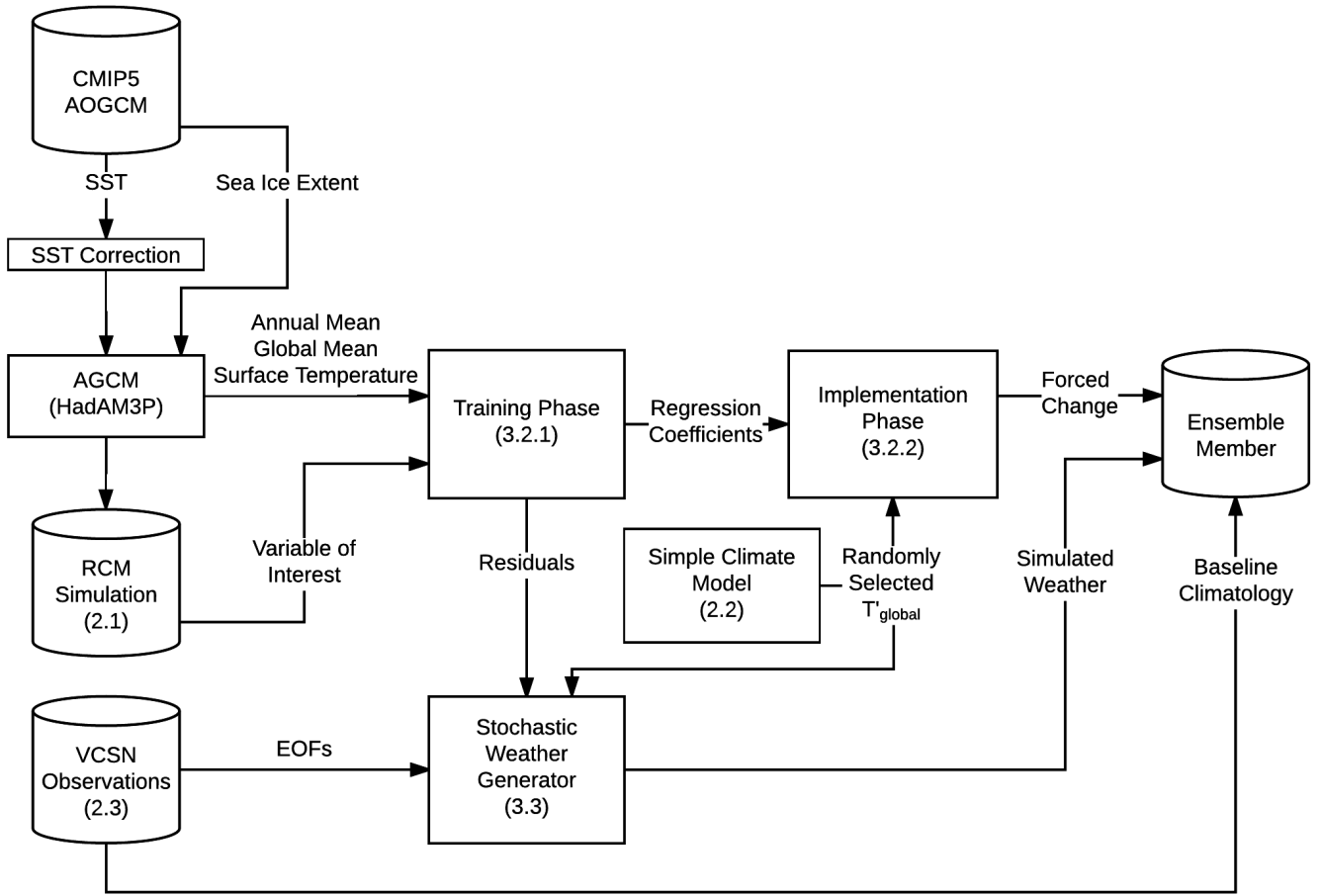
Figure 1. Flow chart illustrating the processes involved in generating a single EPIC ensemble member based on training from a selected RCM simulation. Numbers in brackets refer to the section-Section where more details are provided.
