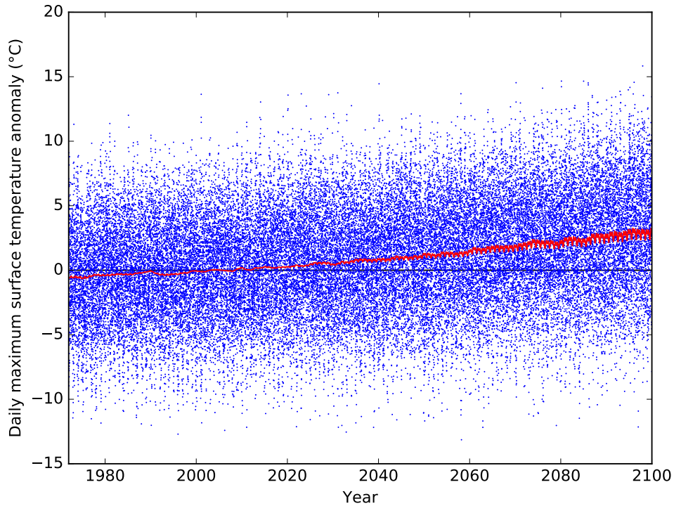
Figure 4. An example of the fit of Eq. (32) (red line) to daily maximum surface temperature anomalies (blue) obtained from the NorESM1-M RCM simulation under the RCP8.5 GHG emissions scenario at Alexandra, New Zealand ( 45.249^{\circ}\text{S} , 169.396^{\circ}\text{E} ). Solid line represents the zero line (no change).
