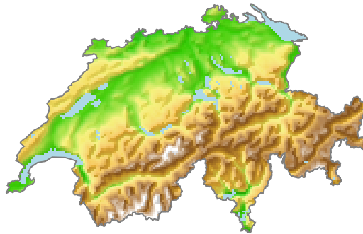
Figure 1. Top: configuration of the four nested domains used in both the WRF-ERA and WRF-CESM simulations. Bottom: detail of the actual orography implemented in the 2-km resolution simulation over Switzerland.
