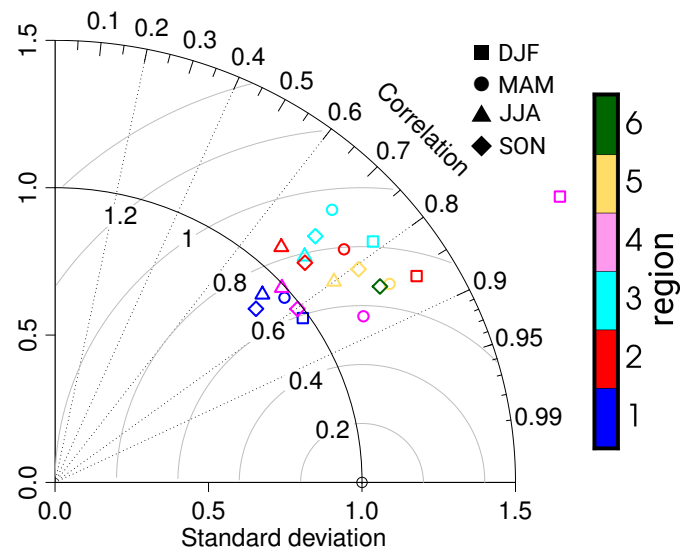
Figure 4. Taylor diagram showing the temporal correlation and ratio of standard deviation between the regional series in the WRF-ERA simulation and the observations across all 4 seasons. For obtaining the regional series, the regions defined for WRF-ERA are used in both datasets. Different symbols denote the result for each season, whereas the colours correspond to the different regions according to the legend and spatial structure shown in middle column in Fig. 2.
