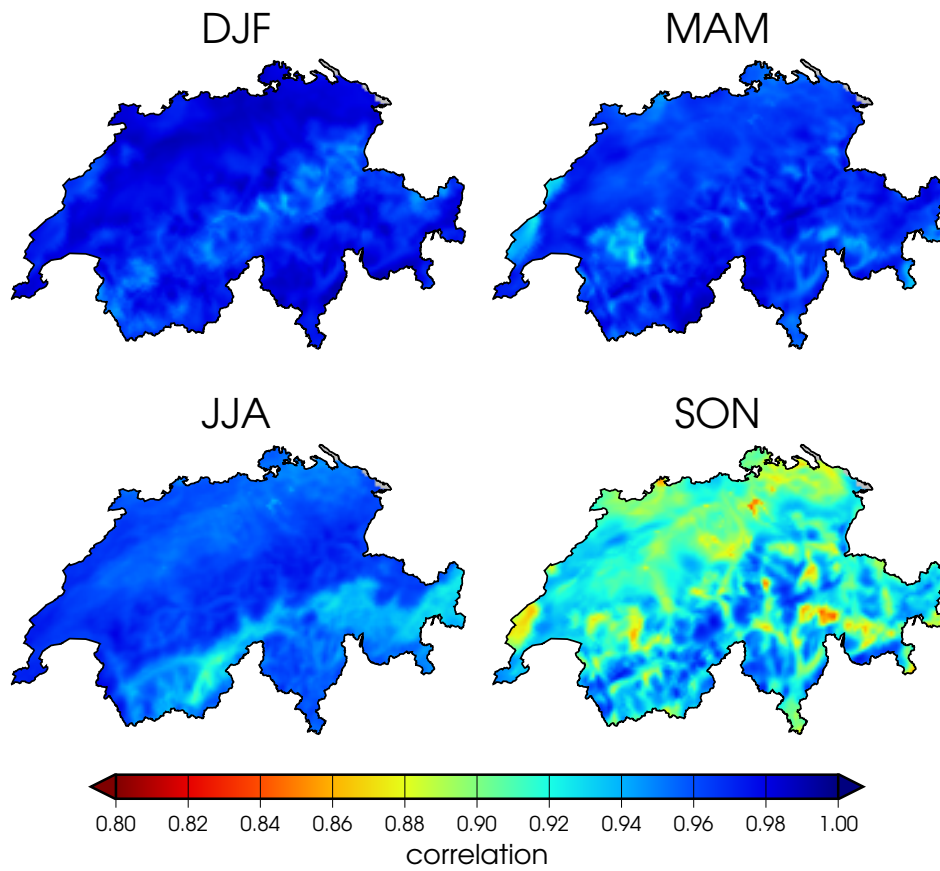
Figure 8. Correlation maps between the daily series of precipitation in the raw WRF-CESM simulation and the output of the bias corrected. The analysis is carried out separately by seasons to minimize the effect of the annual cycle on correlation.
