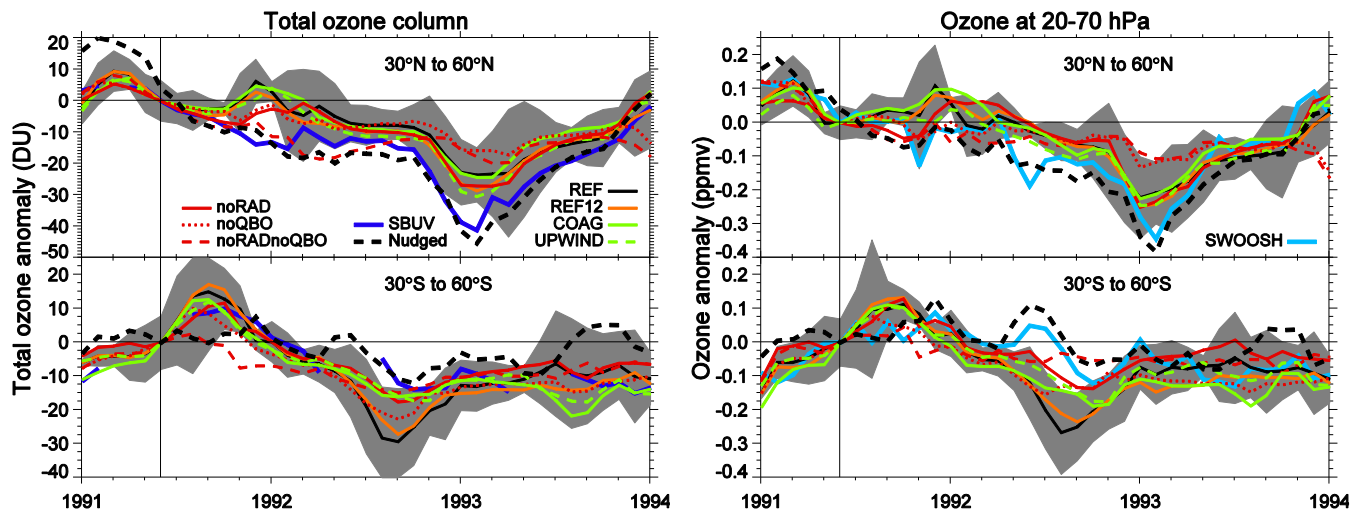
Figure 8. Monthly mean midlatitude ozone ( 30^{\circ} - 60^{\circ} north and south) ozone anomalies from SOCOL-AER compared with observations. Left panels: total ozone column. Right panels: ozone mixing ratio at 20-70 hPa. Observational data sets SWOOSH and SBUVv8.6 are denoted by light and dark blue lines, respectively. Anomalies are computed by subtracting the annual cycle. Grey shaded area: 2\text{-}\sigma ensemble spread of the REF experiment. All other experiments are shown as ensemble means.
