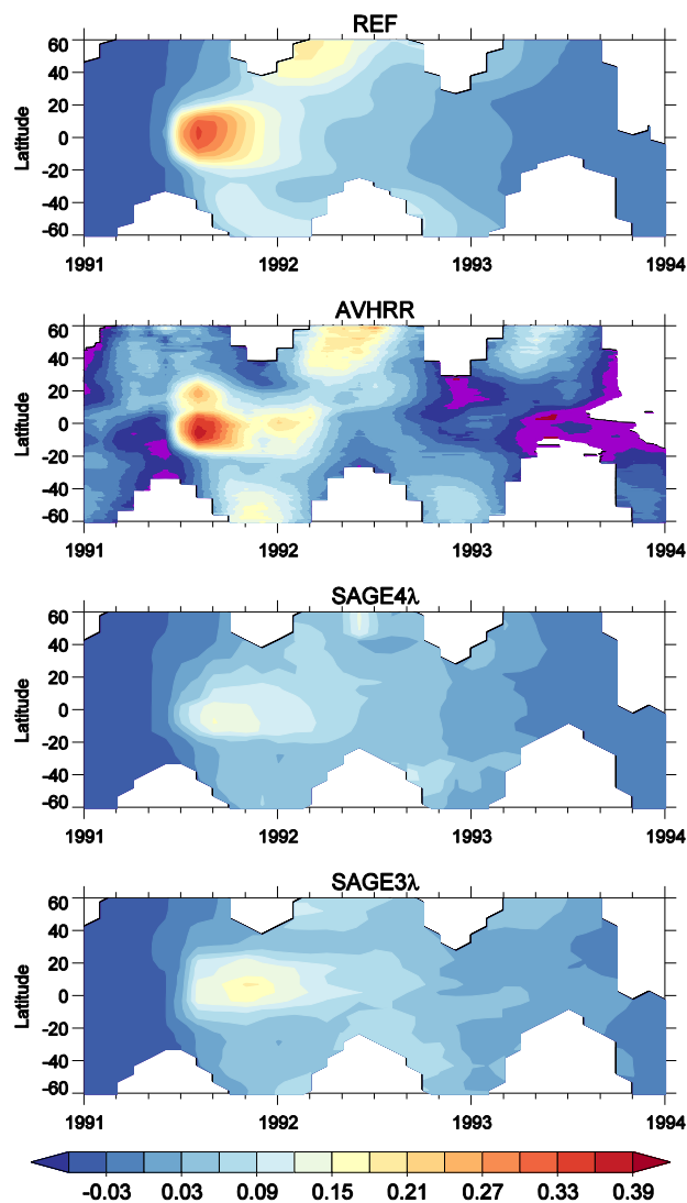
Figure 4. Monthly zonal average total AOD measured at 0.63 \mu\text{m} by AVHRR and calculated at 0.56 \mu\text{m} above tropopause by SOCOL-AER and provided by SAGE3,4 \lambda composites. Since AVHRR measurements were performed over oceans, we applied the same selection for the model here. SAGE3,4 \lambda data were, however, initially provided as zonal means. Background values are subtracted from all data sets (which may result in slightly negative values). All panels are masked at winter high latitudes where AVHRR data are missing.
