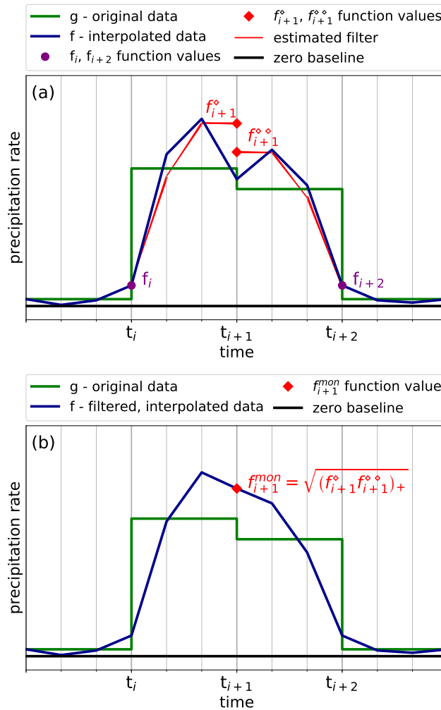
Figure 8. Illustration of the monotonicity filter construction. The original precipitation rate g is shown in green with a 3-hourly resolution. The IA0 interpolated data f on the new sub-grid with 1-hourly resolution is given in dark blue. A zero baseline is shown in black. (a) At first the function value f_{i+1} is split in f_{i+1}^{\diamond} and f_{i+1}^{\circ} shown as red squares. Other function values are recomputed as shown with the red line where f_i and f_{i+2} remain unchanged as shown with purple circles. (b) Second, the function value f_{i+1} is substituted by the new function value f_{i+1}^{mon} as marked with a red square.
