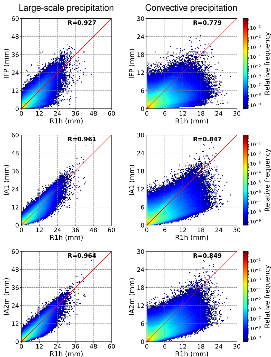
Figure 16. Two-dimensional histogram (relative frequencies) showing the relationship between the hourly precipitation reconstructed by (a) IFP, (b) IA1 and (c) IA2m and the true R1h precipitation, based on the global data set for the year 2014. For each axis, 100 equally-distributed bins were used. The correlation coefficient is annotated to each plot, and the one-to-one line is shown in red.
