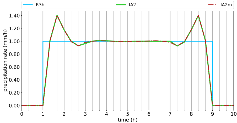
Figure 12. Same as Figure 11, but comparing only IA2 and the modified version IA2m. It is recommended to zoom in to see the differences clearly.
