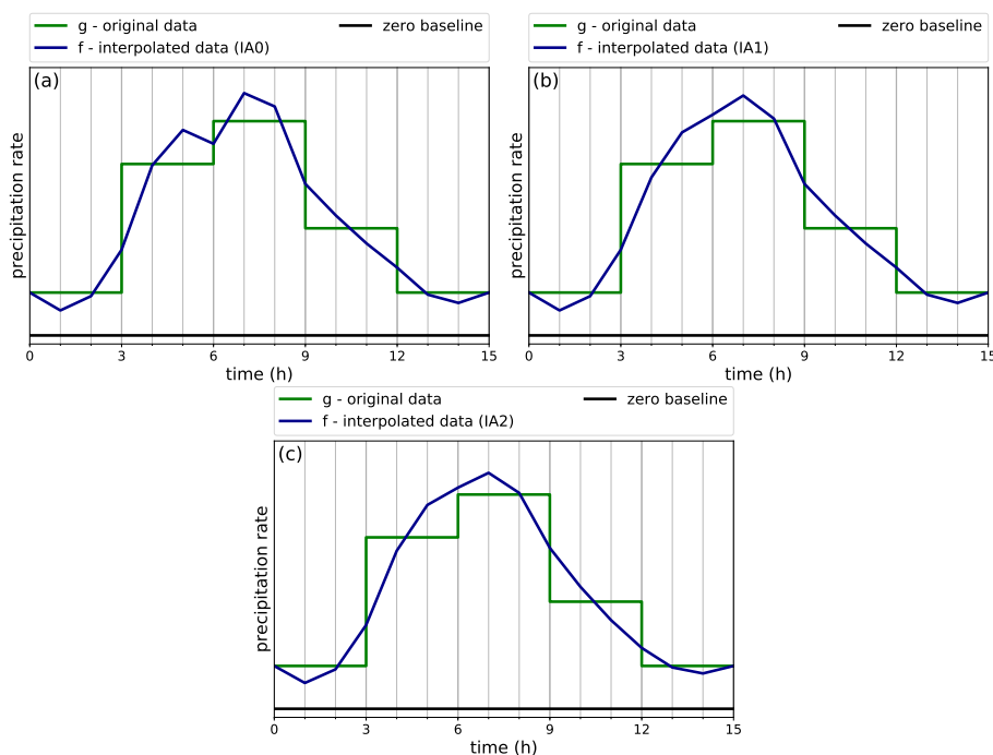
Figure 9. Illustration of the basic IA0 algorithm in (a), with the additional monotonicity filter in algorithm IA1 in (b) and the directly implemented filter in the algorithm IA2 in (c). The original precipitation rate g is shown in green with a 3-hourly resolution. The IA0 interpolated data f on the new sub-grid with 1-hourly resolution is given in dark blue. A zero baseline is shown in black.
