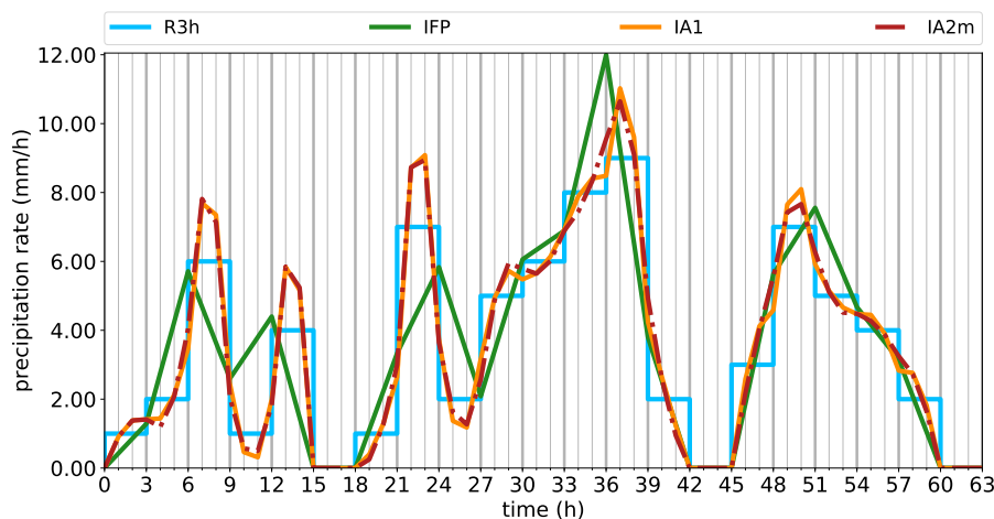
Figure 13. Verification of the different behaviour of the interpolation algorithms for a complex synthetic precipitation time series. R3h is the input data series with 3 h resolution, IFP is the linearly interpolated curve according to the current scheme in FLEXPART, while IA1 and IA2m are the reconstructions using the new algorithms.
