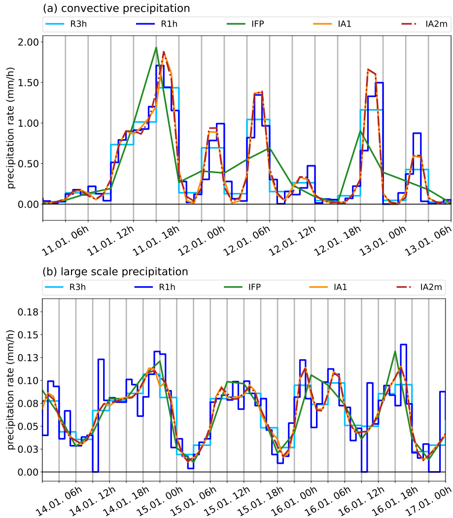
Figure 14. Sample periods in January 2014 at the grid cell centred on 48°N, 16.5°W. (a) 11 Jan 00 UTC to 13 Jan 06 UTC for convective precipitation intensity, and (b) 14 Jan 00 UTC to 17 Jan 00 UTC for large-scale precipitation intensity. Original ECMWF data are shown as step functions (1-hourly: R1h, 3-hourly: R3h), while the interpolation resulting from the reconstructions algorithms (new algorithms: IA1 and IA2m, current FLEXPART algorithm: IFP) are piecewise linear between the respective supporting points. A baseline is drawn in black at intensity value zero.
