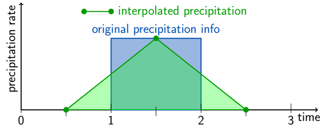
Figure 1. Illustration of the basic problem using an isolated precipitation event lasting one time interval represented by the thick blue line. The amount of precipitation is given by the blue-shaded area. Simple discretisation would use the green circles as discrete grid-point representation and interpolate linearly in between, indicated by the green line and the green-shaded area. Note that supporting points for the interpolation are shifted by a half time interval compared to the times when other meteorological fields are available.
