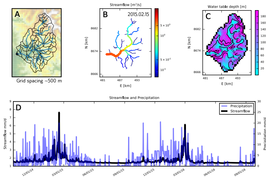
Figure 5. Model based on Río Shullcas, Peru. (A) Map with MODFLOW grid, HRU outlines, stream segments (blue), and digital elevation model. (B) Streamflow accumulation through the mountainous drainage network. (C) The modeled water table distribution with elevation contours (m.a.s.l.). (D) Seasonally variable precipitation and streamflow.
