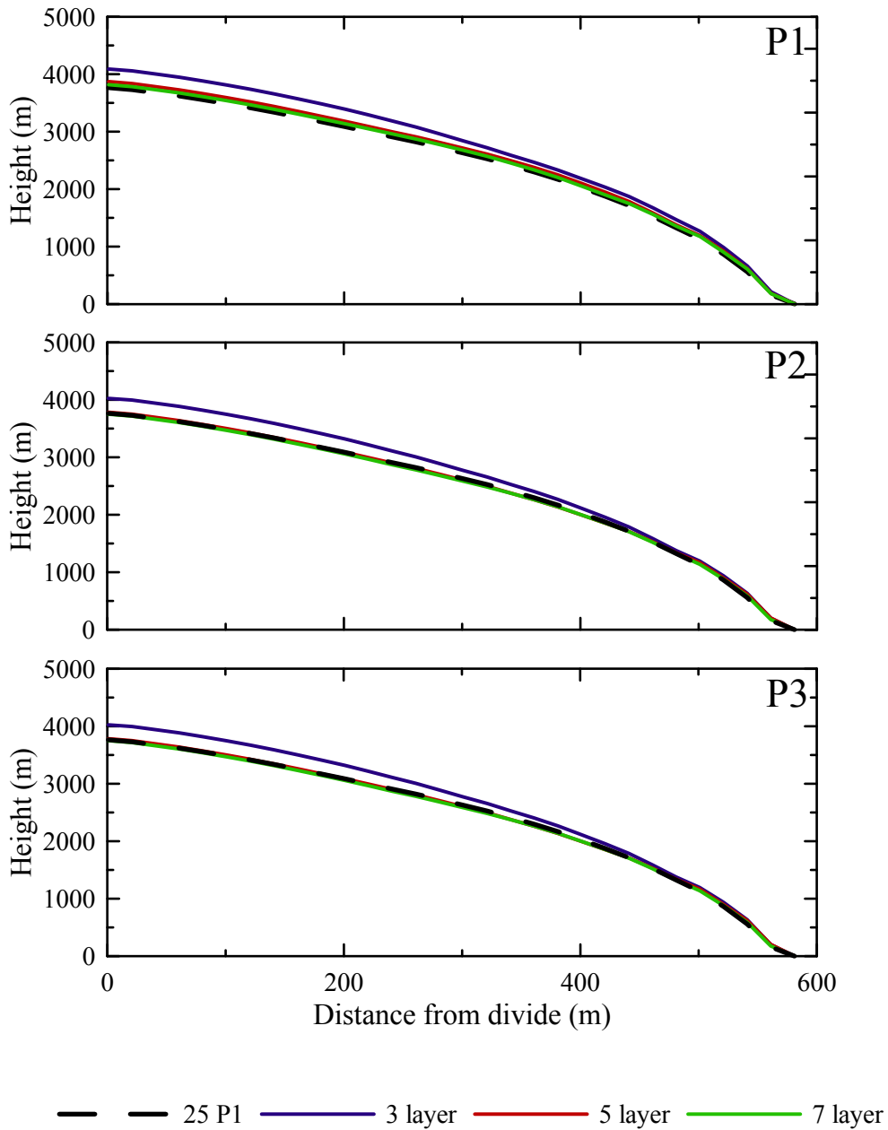
Figure S1. Profiles of ice thickness for models with 3, 5, and 7 layers compared to the 25 layer P1 model simulation at the end of the 100,000 year relaxation for the ice dome experiment.
