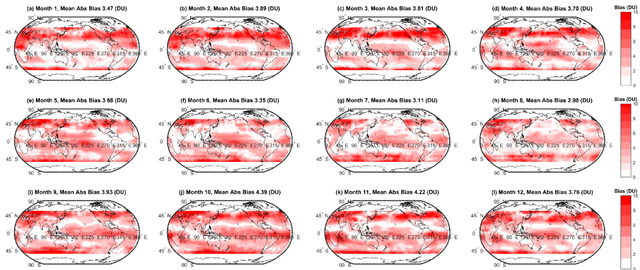
5 Figure 5. Monthly absolute bias (DU) between the simple arithmetic multi-model mean (MMM) tropospheric ozone column and the observed climatology.
