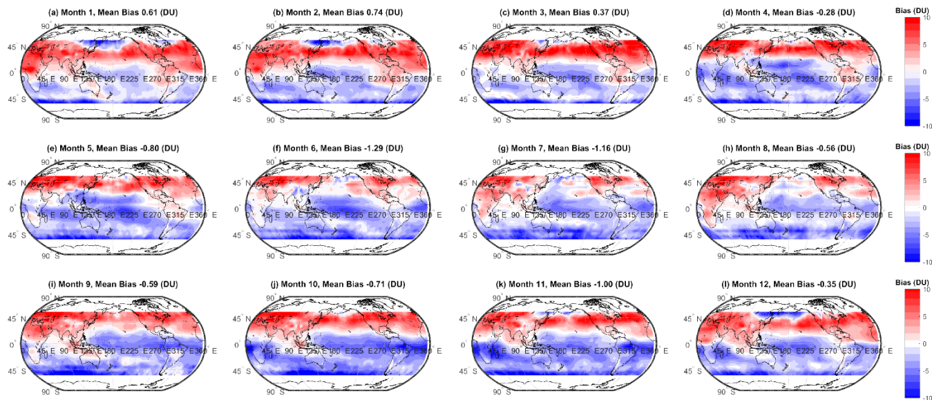
Figure 3. Monthly bias (DU) between the simple arithmetic multi-model mean (MMM) tropospheric ozone column and the observed climatology.
