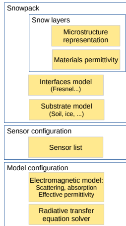
Figure 2. SMRT architecture and main components. The core components (blue) are fixed and contains no scientific code in contrast to the switchable and extensible components (orange) which define the snowpack and model configurations.
