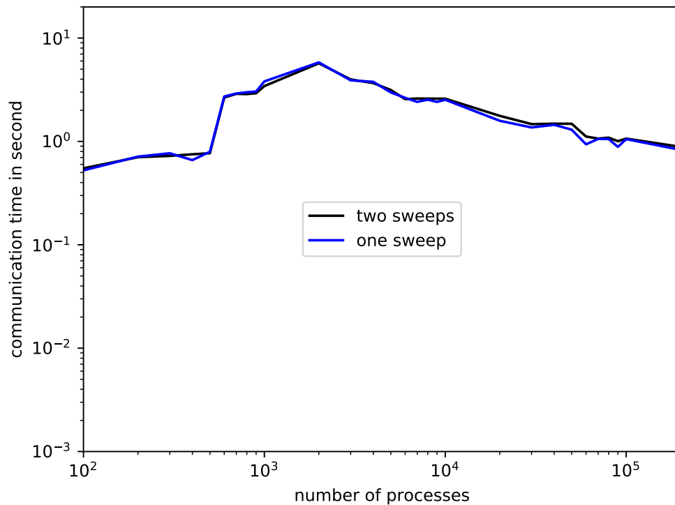
Fig. 1. Communication times of wide halo exchange between the two sweep method and the single sweep method
