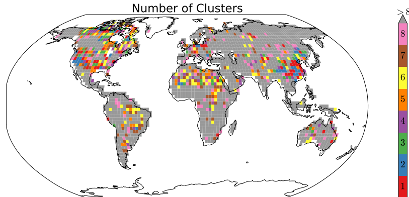
Figure A4. Global distributions of the number of clusters (tiles) found per CLASS-CTEM grid cell when minPts (see Section 2.3) is set to 1% of the number of GSDE data points in the CLASS-CTEM gridcell. The gray regions have >8 tiles found by the clustering algorithms.
