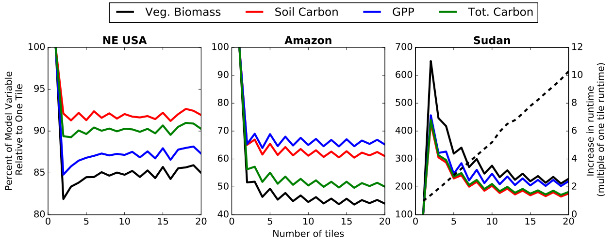
Figure 1. Sensitivity test of CLASS-CTEM to the number of tiles (clusters) for three test grid cells. The texture of each tile as the number of tiles increases is described in Section 3.1. GPP is gross primary productivity. All simulations were run until a new equilibrium state was established. The increase in runtime of the model is displayed as a dashed line.
