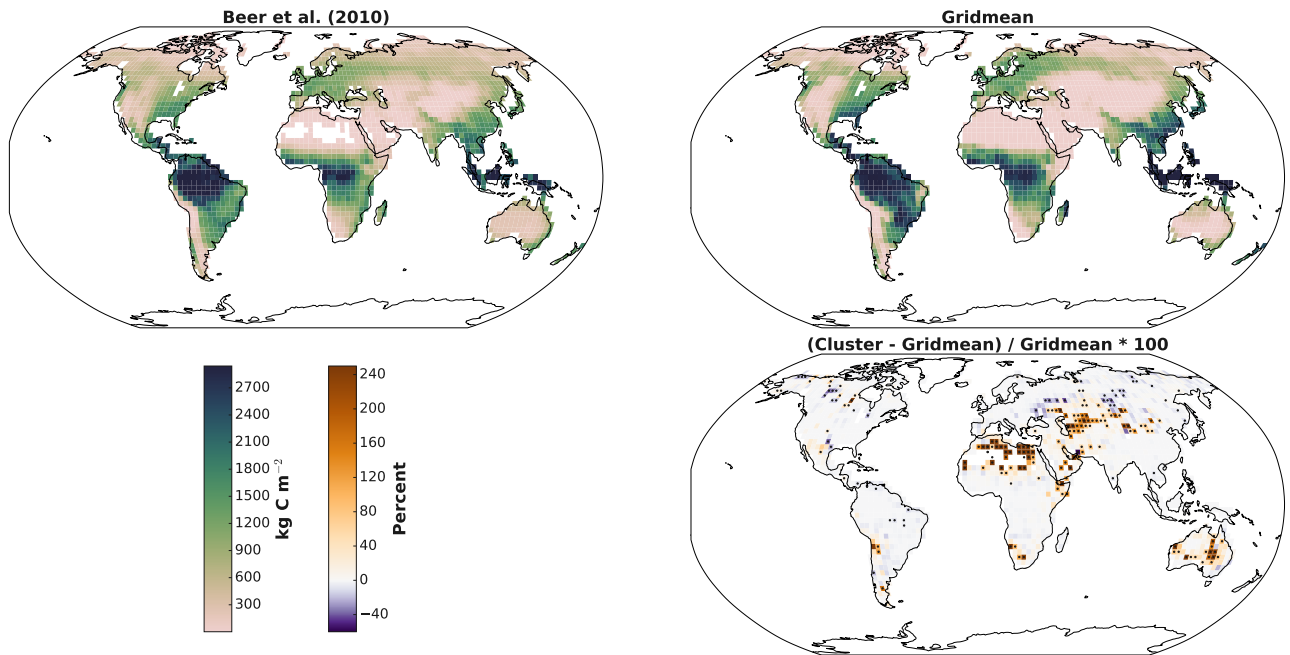
Figure 8. Mean annual gross primary productivity (1982 – 2008) from an observation-based dataset (?) (top left), the Gridmean simulation (top right), and percent relative difference between the Cluster and Gridmean simulations (bottom right). Note that many of the regions with the largest changes in GPP between the two approaches are also regions with low GPP hence the absolute change in GPP is generally small. Dots indicate grid cells that are statistically significant (independent two sample t-test p-level <0.01). For the areas of significant change in GPP between the Cluster and Gridmean simulations, comparison of Cluster and Gridmean simulations against observations was not significant after accounting for the observational uncertainty.
