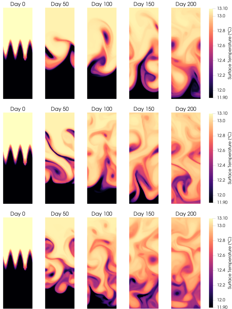
Figure 5. Sea surface temperature fields for the eddy channel test case at 4 km horizontal mesh resolution. Horizontal viscosity is 200 (top row), 50 (middle), and 20 \text{ m}^2 \text{ s}^{-1} (bottom). These values correspond to mesh Reynolds numbers 2, 8, and 20, respectively.
