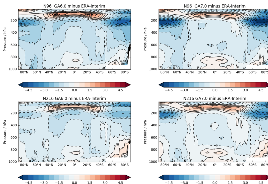
Figure 17. Annual mean zonal mean temperature biases (K) versus ERA-interim in the 27 year N216 atmosphere/land-only climate simulations presented in Fig. 12, alongside results from equivalent simulations performed at N96 resolution. The rows show data from N96 (top) and N216 (bottom), whilst the columns are data from GA6.0 (left) and GA7.0 (right).
