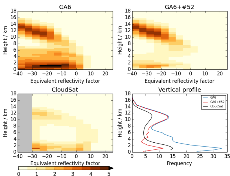
Figure 2. Histograms of height vs 94 GHz radar reflectivity over a trade cumulus region ( 130\text{--}160^\circ\text{W} , 0\text{--}20^\circ\text{S} ), showing climatologies of CloudSat observations and simulated CloudSat data from 20 year N96 atmosphere/land-only climate simulations using GA6.0 and GA6.0 plus the new warm microphysics scheme.
