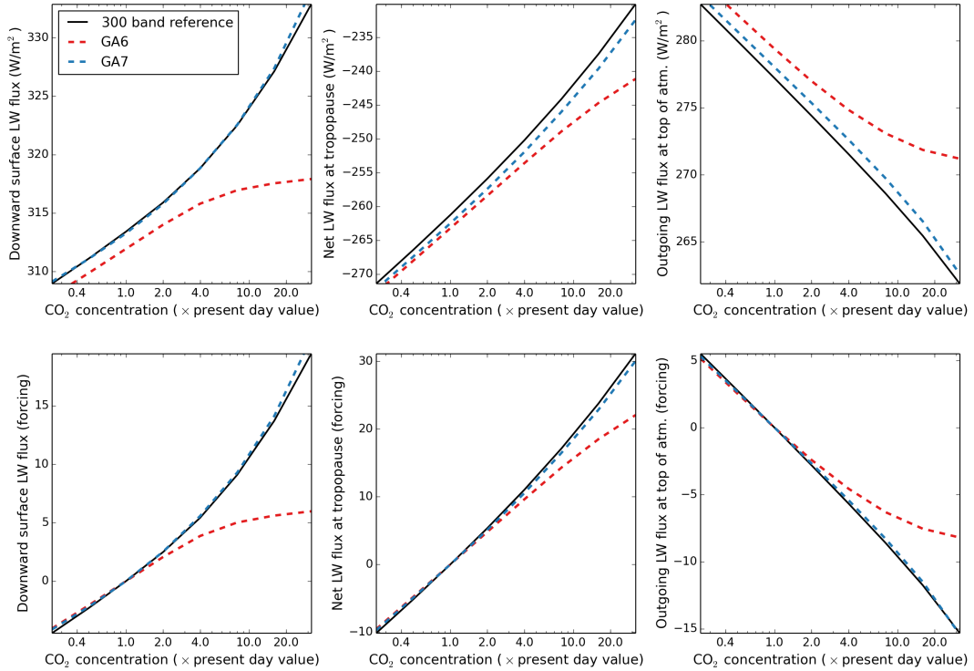
Figure 1. Comparison of LW flux errors due to changes in CO 2 concentration using GA6 and GA7 gaseous absorption compared to a 300 band LW reference configuration. Plots show an average response over the four clear-sky atmospheric profiles used for CIRC (Oreopoulos et al., 2012) which represent a broad range of water vapour path lengths. The top row shows the actual mean fluxes over the four profiles, whilst the bottom row shows the flux differences compared to a run using present day CO 2 .
