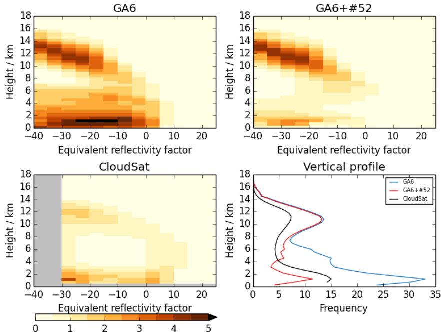
Figure 2. Histograms of height vs 94 GHz radar reflectivity over a trade cumulus region (130–160°W, 0–20°S), showing climatologies of CloudSat observations and simulated CloudSat data from 20 year N96 atmosphere/land-only climate simulations using GA6.0 and GA6.0 plus the new warm microphysics scheme.
