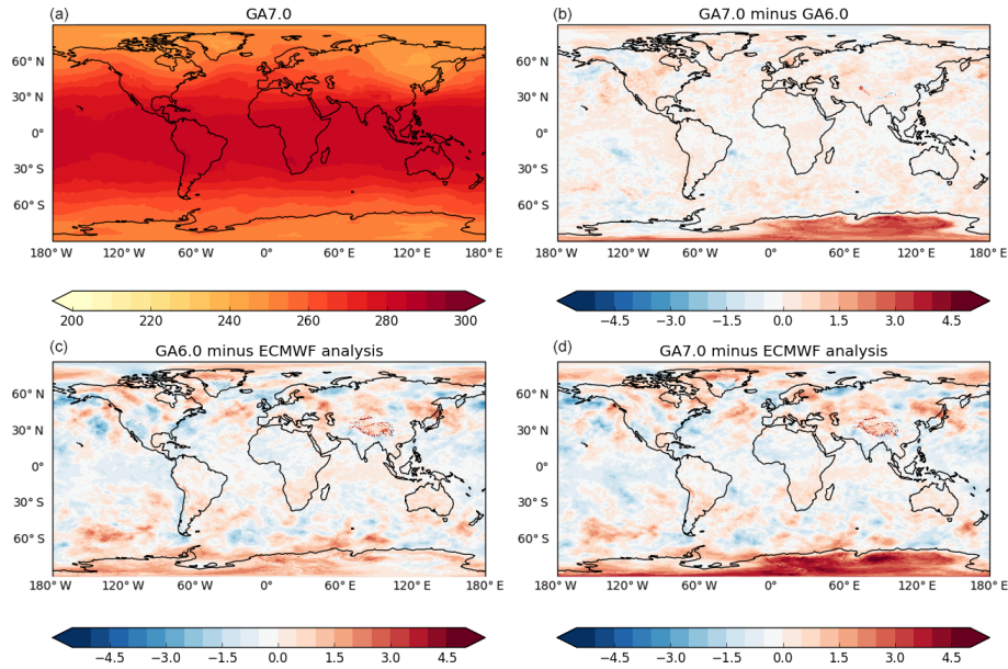
Figure 24. T+120 temperature (K) at 700 hPa mean over the 12 pairs of forecasts included in Fig. 21 that were initialised in DJF. The panels show the mean GA7.0 forecast (a), the difference between GA7.0 and GA6.0 forecasts (b), and the bias compared to the verifying ECMWF analyses in GA6.0 (c) and GA7.0 (d).
