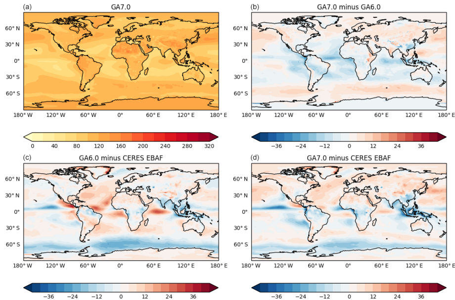
Figure 15. Annual mean top-of-atmosphere reflected SW radiation ( \text{W m}^{-2} ) in the 27-year N216 atmosphere/land-only climate simulations presented in Fig. 12 compared to Earth's Radiant Energy System (CERES) Energy Balanced and Filled (EBAF) dataset (Loeb et al., 2009). The layout is the same as in Fig. 13.
