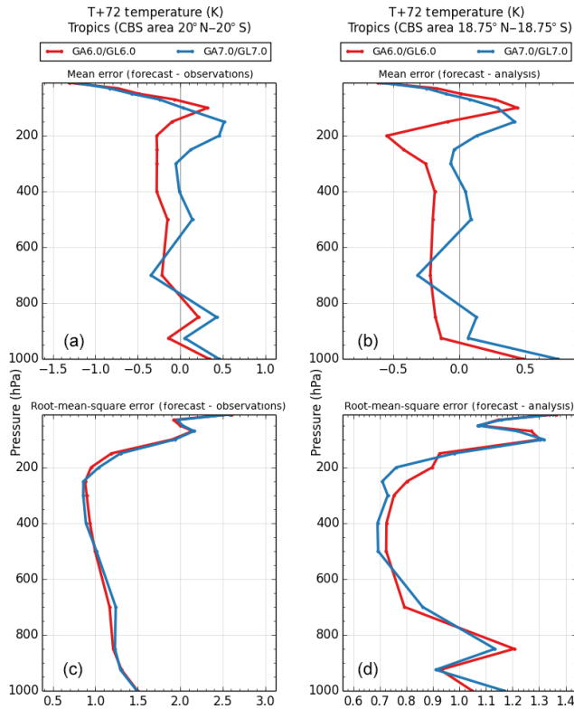
Figure 22. Profiles of 3-day (T+72) tropical temperature bias (a, b) and RMSE (c, d) T S2 versus radiosonde observations (a, c) and ECMWF analyses (b, d) from the N768 GA6.0 and GA7.0 case studies presented in Fig. 21.
