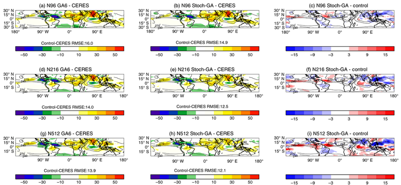
Figure 11. Mean June–August (JJA) top-of-atmosphere outgoing LW radiation (OLR) errors ( \text{W m}^{-2} ) from 20-year atmosphere/land-only climate simulations compared to Earth's Radiant Energy System (CERES) Energy Balanced and Filled (EBAF) dataset (Loeb et al., 2009). The columns from left to right are GA6.0 controls, GA6 plus the stochastic physics package (labelled Stoch-GA) and the difference between the two, whilst the rows from top to bottom are from simulations at N96, N216 and N512 resolution. This figure is reproduced from Sanchez et al. (2016).
