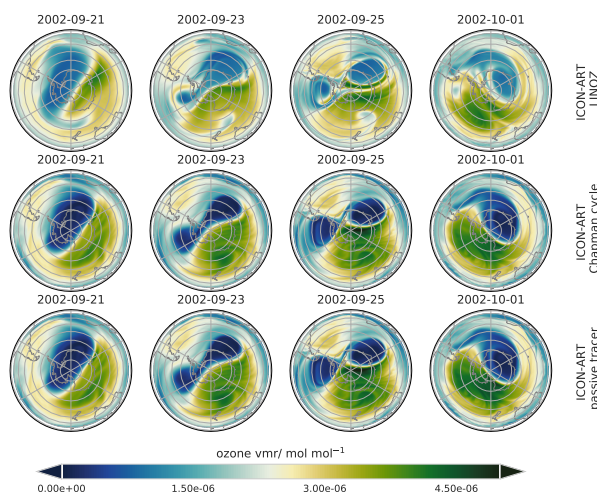
Figure 4. Passive and active ozone tracers [ \text{mol mol}^{-1} ] at 50 hPa over Antarctica. Daily averages for two ICON-ART simulations for the Linoz chemistry scheme (top) and for the extended Chapman cycle chemistry (mid) and the passive tracer (bottom) are shown.
