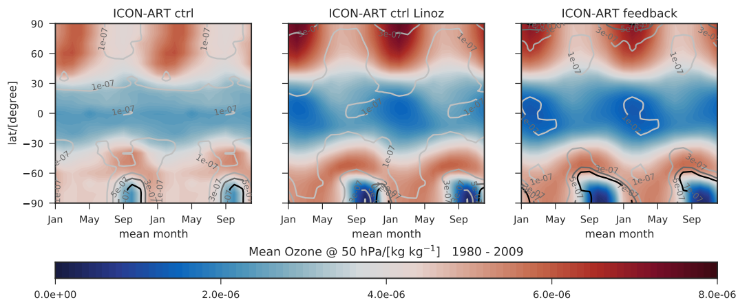
Figure B1. Monthly averaged zonal means of ozone [ kg\ kg^{-1} ] at 50 hPa (shown twice) for the period from 1980 to 2009 (shaded). Contour lines represent the standard deviation of the monthly means. Left panel: ozone climatology as used in the control simulation; middle panel: non-interactive Linoz ozone; right panel: interactive Linoz ozone.
