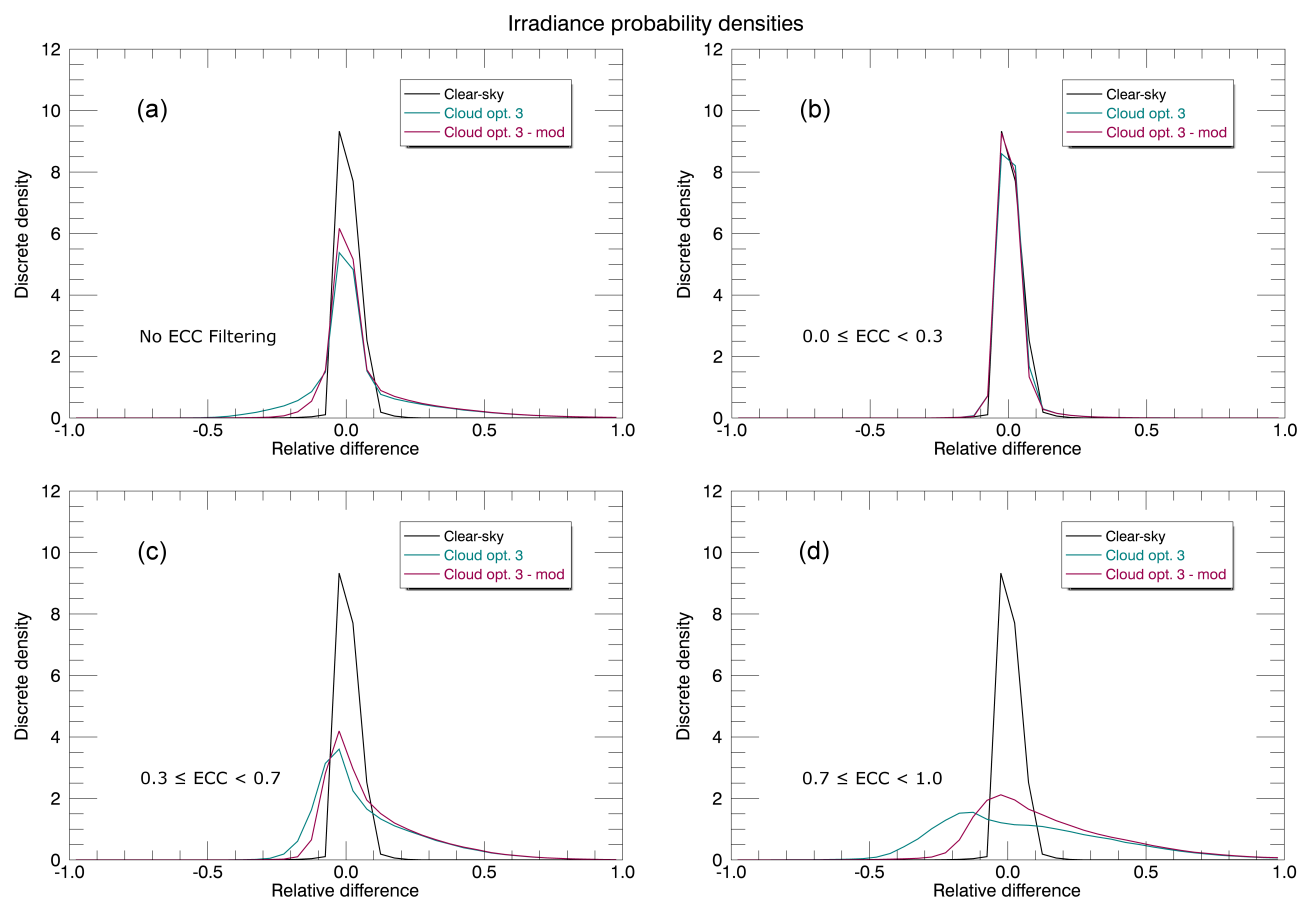
Figure 13. Irradiance probability density plots demonstrating the dependence of the 330-400 nm surface irradiances on cloud cover (ECC). Plotted are the relative differences between the Cloud-J and GEM surface irradiances under unattenuated, clear-sky conditions (black), cloudy-sky where the Cloud-J Option 3 cloud flag is used to calculate cloud attenuation (green), and a modified version of the GEM model output for cloudy skies compared to the Cloud-J data employing the Option 3 cloud flag (purple). The modification made to the GEM code was to change the effective radii for the ice clouds to determine if it made any difference relative to the Cloud-J output. In all four plots, a solar zenith angle filter was applied, where only surface irradiances pertaining to locations where zenith angles <70^\circ are used. A secondary filter for varying total effective cloud cover is employed in the plots to display the relative difference in irradiances for a given range of cloud cover from clear-sky (0.0) to completely overcast (1.0).
