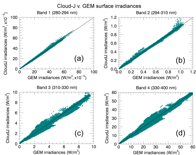
Figure 8. Calibrated GEM broadband, corrected using the total irradiance scaling functions found in Table 1, compared to the simulated GEM broadband produced by Cloud-J.
