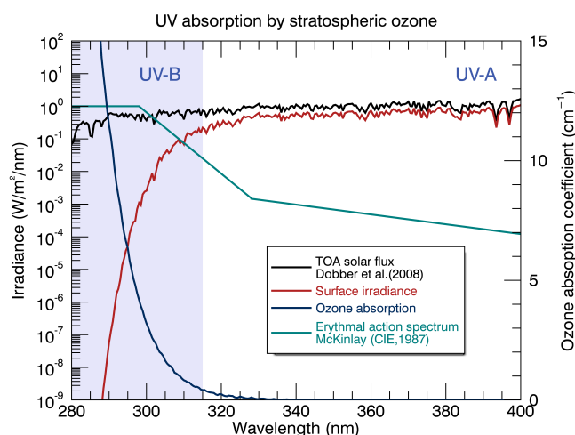
Figure 1. Sample UV irradiance spectrum at the Earth's surface on a clear summer day (averaged and sampled over 0.5 nm intervals). Stratospheric (O 3 ) is the primary species which serves to absorb UV radiation in the atmosphere (blue curve). The Huggins/Hartley band system of O 3 attenuates the radiative flux (black curve) by several orders of magnitude in the UV-B region. The product of the absorption cross-section and the top-of-atmosphere flux gives the resultant incoming irradiance at the surface (red curve). The erythral action spectrum (green curve), demonstrates the increasing susceptibility of human skin to epidermal damage (erythema).
