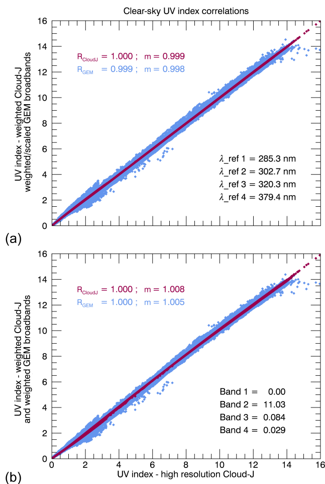
Figure 10. Correlation of the UV Index fields generated from the Cloud-J (purple) and GEM (blue) broadband. Results from the least-squares minimization using the integration approach (upper panel, a) produced reference positions of 285.3, 302.7, 320.3 and 379.4, respectively for each UV sub-bands. Minimization performed using the direct linear fitting method (lower panel, b) produced coefficients of 11.03, 0.084, and 0.029 for bands 2 through 4, respectively, where the weighting for band 1 was intentionally fixed to a value of zero.
