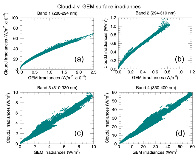
Figure 5. Correlation of GEM and Cloud-J total surfaces irradiances for clear-sky conditions. The GEM UV broadband are compared to simulated broadband produced by integrating the high resolution Cloud-J output over the same spectral regions. Presented are the individual, 7-day irradiance contributions from 23-29 August 2015.
