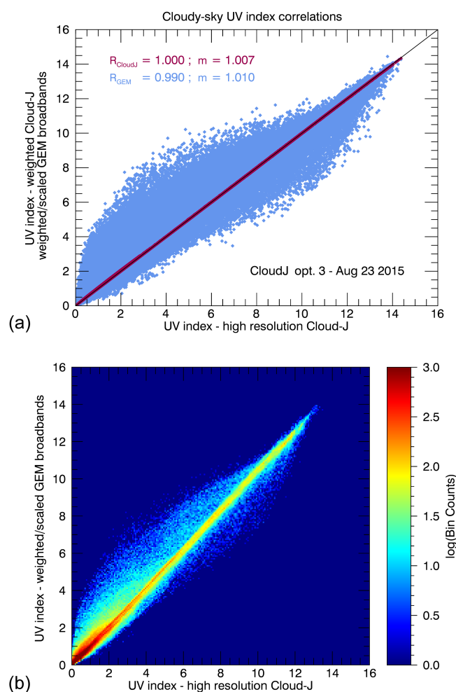
Figure 12. Analogous correlations of the UV Index fields generated from the Cloud-J (purple) and GEM (blue) broadband under cloudy-sky conditions using Cloud-J cloud flag Option 3 in the comparison. The upper panel, a, presents the direct linear correlations of the UV index calculated using the GEM and Cloud-J broadband relative to the high resolution output produced by Cloud-J using the same scaling functions and weighting determined through the integration approach under clear-sky conditions. The lower panel, b, is a density plot of the correlation of the UV index calculated using the GEM broadband compared to the Cloud-J, high resolution, UV index field depicted in the upper panel.
