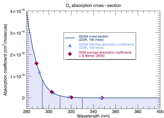
Figure 7. GEISA ozone absorption cross-sections measured at a temperature and pressure of 223 K and 100 mbar, respectively. Overlaid are the effective absorption coefficients calculated from the GEISA cross-section, as described in Sect. 3.1.1, and the GEM average absorption coefficients for each representative UV broadband.
