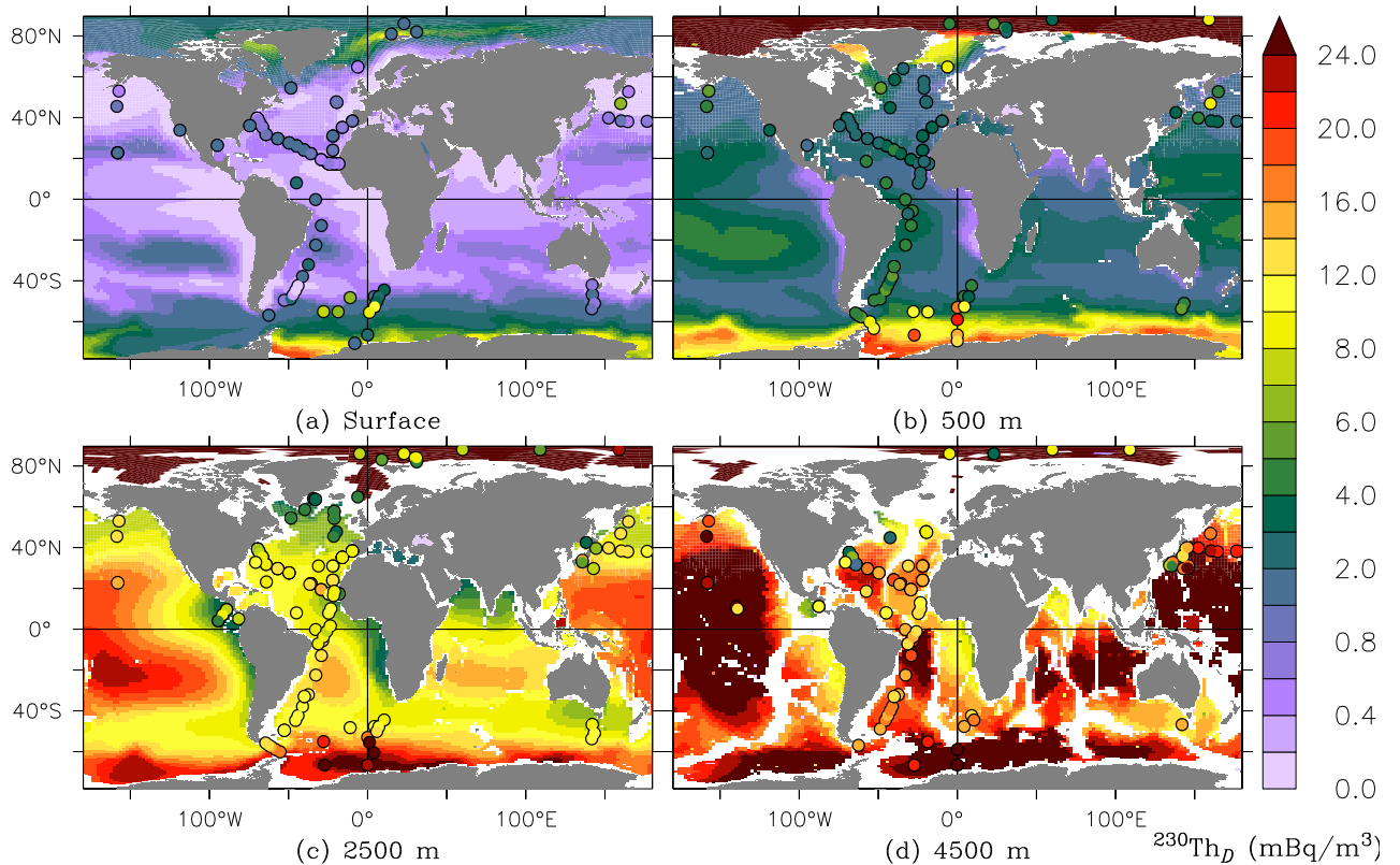
Figure 6. The dissolved thorium-230 activity at four depth levels ( \text{mBq m}^{-3} ), observations as discs at the same colour scale.
