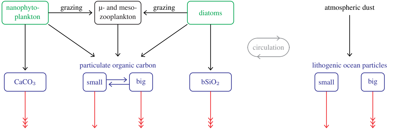
Figure 1. Conceptual model of particle dynamics, on which the numerical model is based. Nanophytoplankton and diatoms (in green) take up nutrients and \text{CO}_2 , which are released again from respiration and remineralisation of bSiO 2 , POC, DOM and lithogenic particles. The nutrients are not represented in the figure, because only particles impact ^{231}\text{Pa} and ^{230}\text{Th} . Zooplankton are denoted by the black box. All sinking particles are denoted by blue boxes. Effectively, this figure comprises the internal cycling of PISCES, minus details that are not of interest here, plus the lithogenic dust model. DOM stands for Dissolved Organic Carbon, sPOM and bPOM stand for small and big Particulate Organic Matter which are both subject to the differential lability scheme (Aumont et al., 2017), and bSiO 2 stands for biogenic silica. Sinking is denoted by the red arrows; triple arrows means fast, normal arrows slow.
