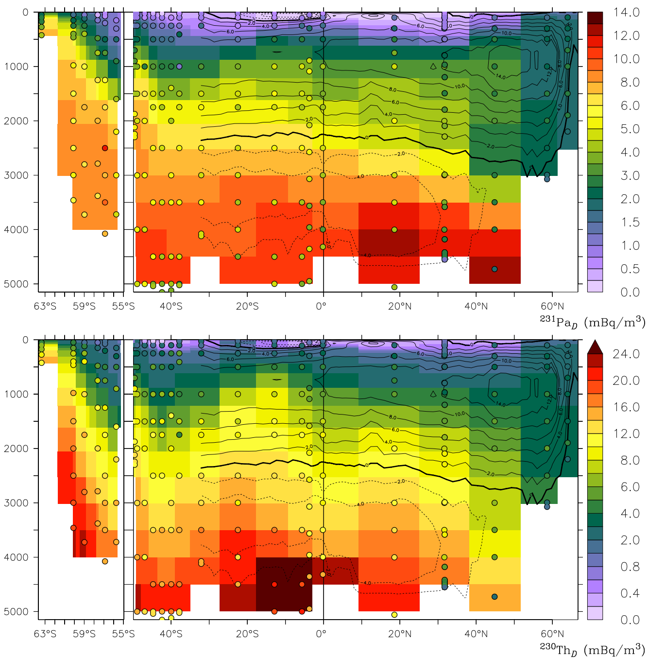
Figure 12. Dissolved protactinium-231 (upper panel), and thorium-230 (lower panel) at the Drake Passage (GIPY5) and West Atlantic (GA02) transects (mBq m -3 ); observations as discs. The Atlantic OSF, in Sv, is superimposed as a contour.
