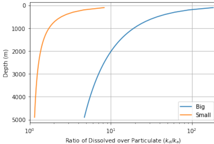
Fig. 1. Ratio of Dissolved to Particulate Isotope
