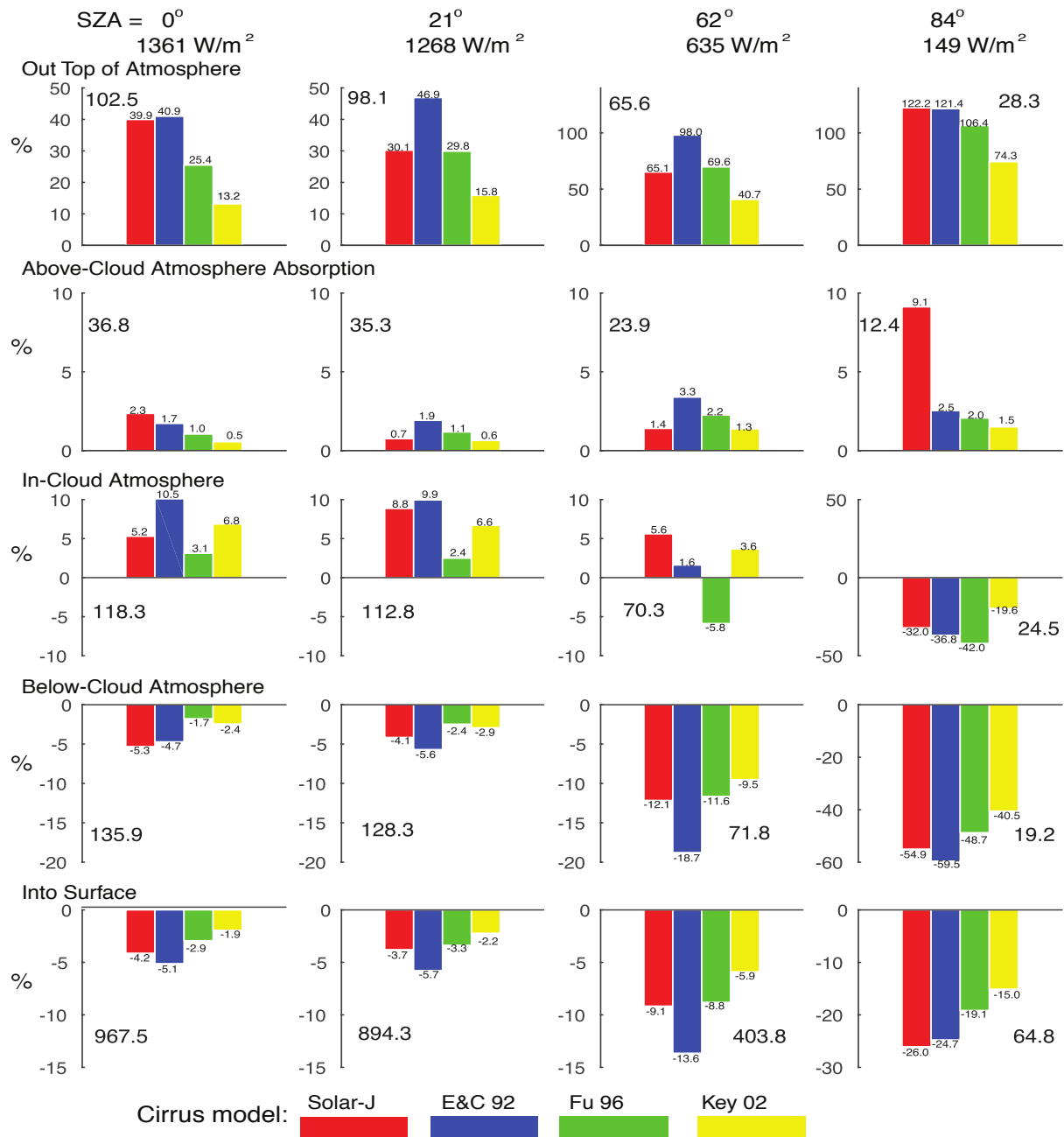
Figure 6. Percent changes (%) in shortwave radiation energy budget relative to the aerosol-free clear sky (surface albedo = 0.06) caused by a cirrus cloud using four different models: Solar-J and the three RRTMG-SW parametrizations for ice clouds. Results are shown for 4 different solar zenith angles. Changes in the vertical column are divided into 5 regions: top of atmosphere, atmospheres above, within and below the cirrus cloud, and at the surface. Single numbers in bold shown in the corner of each panel are the clear-sky energy budget in W m^{-2} averaged over Solar-J and RRTMG-SW for each region. Percentage changes are also shown in text at the end of each color bar. Note that different y-axis scales have been used for large SZAs.
