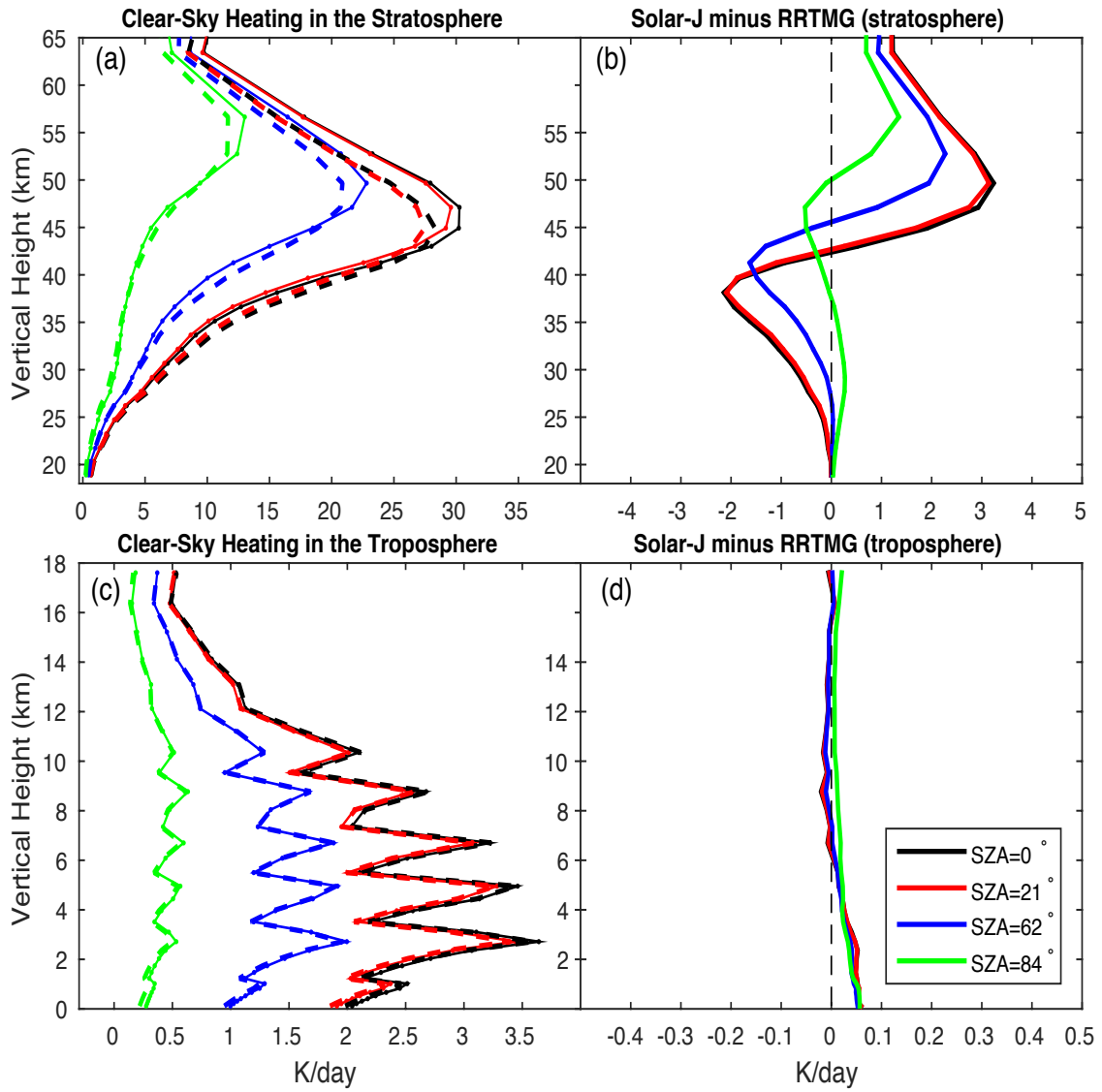
Figure 2 Aerosol-free cloudless atmospheric heating profiles of Solar-J (solid lines) and RRTMG-SW (dashed lines) and the difference, Solar-J minus RRTMG, for a typical July tropical atmosphere at 4 solar zenith angles with Lambertian surface albedo = 0.06 (left and right sides). The plot is further split into the stratosphere and the troposphere (top and bottom rows). Note that the scale of the x-axis, K/day, is 10 times larger for the stratosphere on the top panels.
