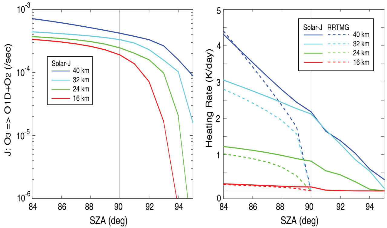
Figure 3: Ozone photolysis rates ( J_{O_3} ) from Solar-J (left panel) and the corresponding atmospheric heating rates under clear sky (right panel) from Solar-J (solid lines) and RRTMG-SW (dashed lines) for large solar zenith angles at 4 different altitudes. RRTMG's heating rates reduce to zeros at SZA= 90° due to the lack of sphericity correction in the plane-parallel approximation; whereas the impact of sphericity on the direct solar beam path is included in Solar-J.
