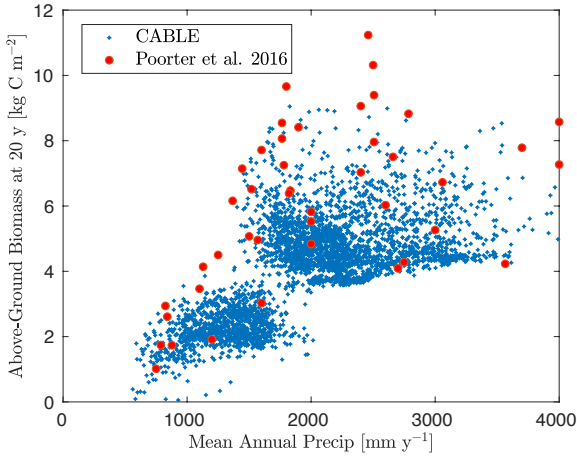
10 Figure 5: CABLE and observation-based estimates (Poorter et al., 2016) of Neotropical secondary forest biomass after 20 years of regrowth versus mean annual precipitation. CABLE estimates are extracted from secondary-forest tiles in Tropical Rainforest, Tropical Seasonal Forest and Tropical Dry Forest/Savanna biomes (Figure 2) in South America. The lower distinct cloud of CABLE simulated values corresponds to the Tropical Dry Forest/Savanna biomes.
