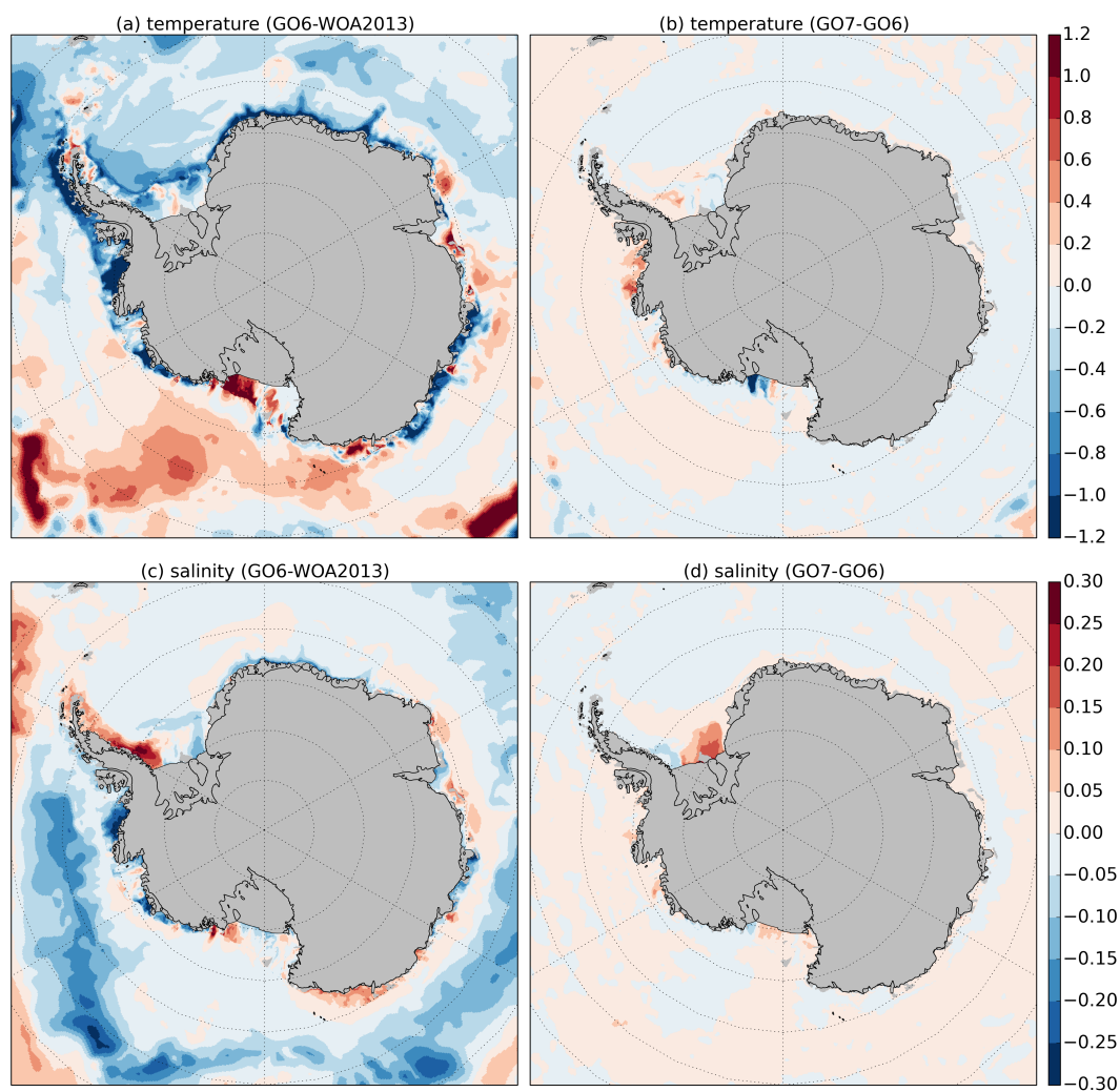
Figure 19. Maps of potential temperature (K) and salinity (psu) averaged between 300 and 1000 m. (a, c) differences between GO6 and WOA2013 (Locarnini et al. (2013) and Zweng et al. (2013)) data; (b, d) differences between GO7 and GO6. Grey shading represents areas covered by ice shelves or ice sheets, or with bathymetry shallower than 300 m.
