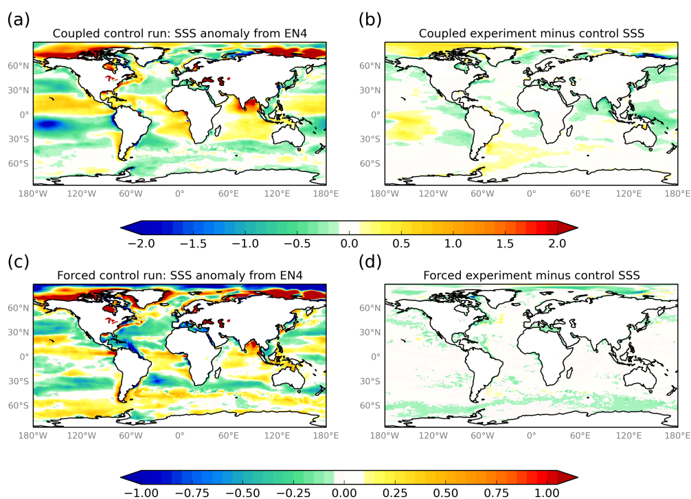
Figure 6. As for figure 5 but for sea surface salinity (psu). Anomalies are against the EN4 analysis (Good et al., 2013).
