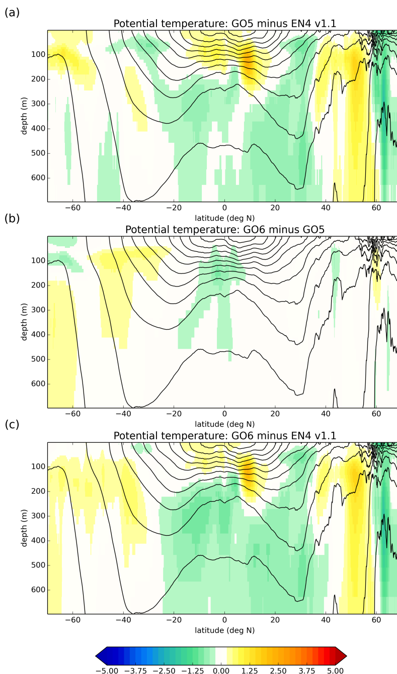
Figure 10. Cross sections of zonal mean potential temperature anomalies (K), showing latitude in degrees on the x-axis and depth in metres on the y-axis. (a) GO5 anomaly against EN4 v1.1 (Good et al., 2013); (b) Difference GO6 minus GO5; (c) GO6 minus EN4 v1.1. Contours are zonal mean potential density \sigma_0 from the GO6 integration with a contour interval of 0.5 \text{ kg/m}^3 . Model fields are time-means over the third decade of the integration.
