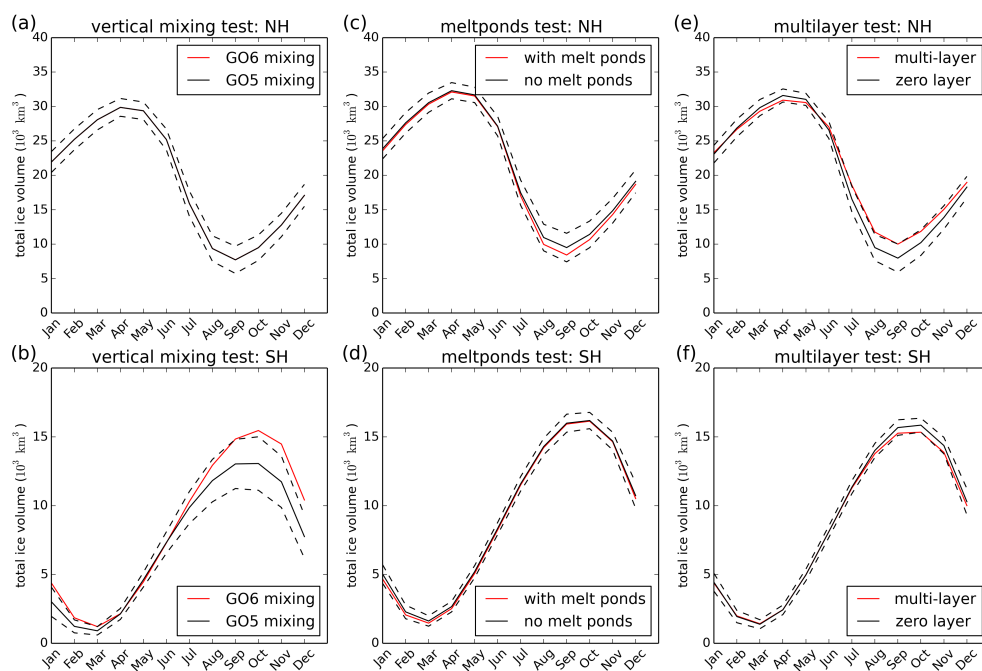
Figure 4. Plots showing the mean seasonal cycle from 10-year forced integrations of integrated sea ice volume for northern hemisphere (top row) and southern hemisphere (bottom row). Results are shown from three sensitivity experiments: (a) and (b) tuning of near-surface vertical mixing; (c) and (d) introduction of explicit calculation of the impact of melt ponds on albedo versus a simple temperature-dependent albedo; (e) and (f) introduction of multi-layer thermodynamics versus zero-layer thermodynamics. In all cases the results with the new settings are in red and with the old settings in black. The dashed lines show the standard deviation of the annual mean values for the control integration in each case.
