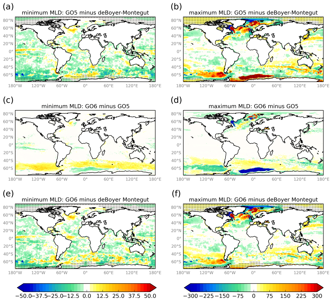
Figure 12. Pointwise minimum and maximum monthly mixed layer depth anomalies (m) and differences in metres calculated as for Figure 3. Hashed regions indicate the presence of sea ice at any time during the year. (a) GO5 minimum monthly mixed layer depth against de Boyer Montégut et al. (2004); (b) GO5 maximum monthly mixed layer depth against deBoyer Montegut; (c) Difference GO6 minus GO5 minimum monthly mixed layer depth; (d) Difference GO6 minus GO5 maximum monthly mixed layer depth; (e) GO6 minimum monthly mixed layer depth against deBoyer Montegut; (f) GO6 maximum monthly mixed layer depth against deBoyer Montegut.
