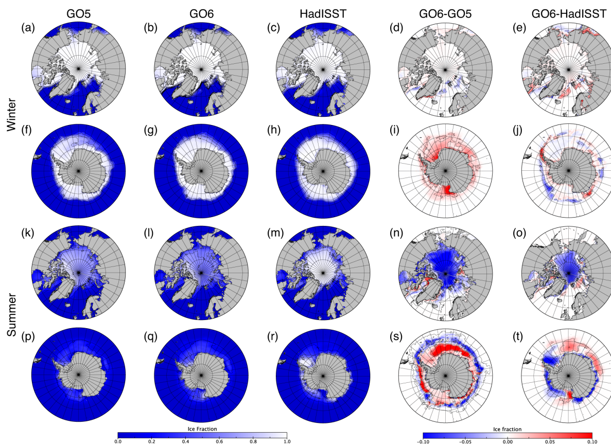
Figure 14. Seasonal-mean multi-annual sea ice concentration for summer and winter, averaged for 1978-2005 in GO5-GSI5.0, GO6-GSI8.1, and the HadISST analysis (Rayner et al., 2003). Panels (a-e) - show GO5-GSI5.0, GO6-GSI8.1 and HadISST ice concentration and the concentration difference between GO6-GSI8.1 and GO5-GSI5.0 and the bias between GO6-GSI8.1 and HadISST respectively for DJF in the Northern Hemisphere (NH); (f-j) are the same as above but for JJA in the Southern Hemisphere (SH); (k-o) are the same as (a-e) but for JJA in the NH; (p-t) are the same as (f-j) but for DJF in the SH.
