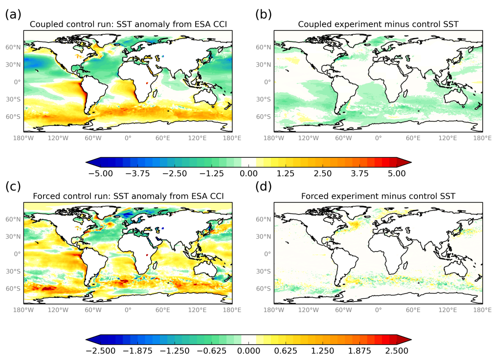
Figure 5. Results from sensitivity tests of halving the isopycnal diffusion parameter (from 300 \text{ m}^2/\text{s} to 150 \text{ m}^2/\text{s} ) in: (a) and (b) the Met Office GC3 coupled configuration (Williams et al., submitted 2017); and (c) and (d) the forced GO6 configuration. Plot (a) shows 15-year mean SST anomalies (K) against ESA CCI (Merchant et al., 2014) from a spin-up of a coupled model with the original diffusion coefficient and plot (b) shows the impact of reducing the isopycnal diffusion parameter. Plots (c) and (d) show the same fields for the second 5 years of a 10-year CORE2-forced GO6 test.
