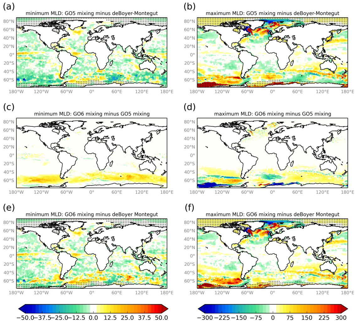
Figure 3. Results from a sensitivity study where the nn\_htau length scale was tuned. A mean monthly climatology of the mixed layer depth field in metres was calculated for the third decade of the spin up (1996-2005). The pointwise minimum and maximum monthly values have then been calculated and plotted as anomalies against the same quantities from the de Boyer Montégut et al. (2004) climatology. Hashed regions indicate the presence of sea ice at any time during the year. (a),(b) minimum and maximum mixed layer depth anomalies for integration with nn\_htau from GO5; (e),(f) as (a),(b) with nn\_htau from GO6; (c),(d) the difference fields between the two integrations.
