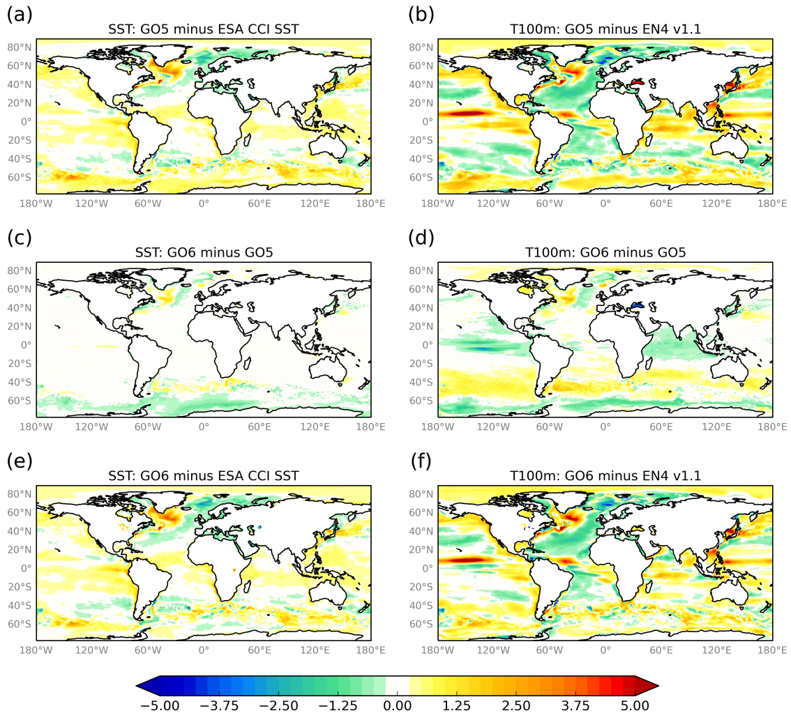
Figure 9. Potential temperature (K): anomalies against climatology and GO6-GO5 differences. (a) GO5 SST anomaly against ESA CCI (Merchant et al., 2014); (b) GO5 100m potential temperature anomaly against EN4 v1.1 (Good et al., 2013); (c) Difference GO6 minus GO5 SST; (d) Difference GO6 minus GO5 100m potential temperature (e) GO6 SST anomaly against ESA CCI; (f) GO6 100m potential temperature anomaly against EN4 v1.1. Model fields are time-means over the third decade of the integration.
