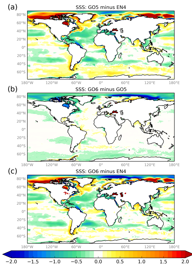
Figure 11. (a) GO5 SSS anomaly (psu) against EN4 v1.1 (Good et al., 2013); (b) Difference GO6 minus GO5 SSS; (c) GO6 SSS anomaly against EN4 v1.1. Fields meaned over the last 10 years of the 30 year spin up.
