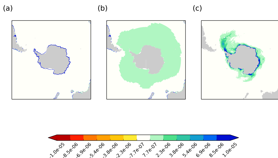
Figure 7. Annual mean freshwater input ( \text{kg/m}^2/\text{s} ) from Antarctic land mass to ocean: (a) Annual mean freshwater input where freshwater input from Antarctica is represented as runoff close to the coastline; (b) as for (a) but with the freshwater input from Antarctica spread over the Southern Ocean to crudely represent iceberg melt; (c) Annual mean freshwater input from Antarctica using the ice shelf parametrization and interactive icebergs scheme.
