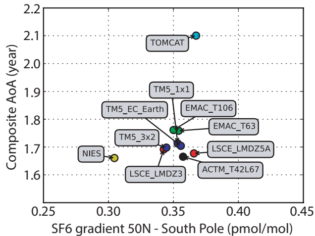
Figure 7. Composite AoA (years) plotted against the modelled SF 6 gradient. The composite AoA is calculated as the sum of the 50°N AoA of tracer "SHsurface" and the 50°S AoA of tracer "NHsurface". The SF 6 gradient is taken as the concentration difference between 50°N and the South Pole from the middle panel of Figure 6. Results are averaged over 2000–2010 (11 years).
