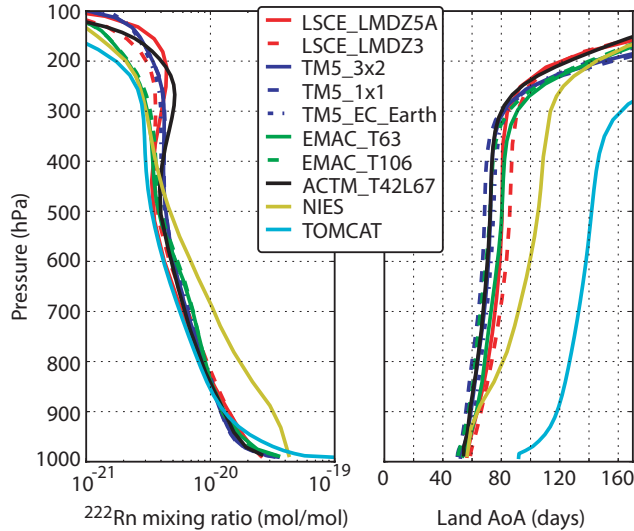
Figure 8. Vertical profiles of ^{222}\text{Rn} (left, \text{mol mol}^{-1} , logarithmic axis) and the AoA of the "land" tracer (right, in days) simulated by the different models. The vertical profiles have been area-weighted-averaged between 60^\circ\text{N} and 60^\circ\text{S} and over the years 2000-2010 (11 years).
