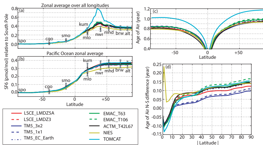
Figure 6. Panels (a) and (b): Latitudinal gradient of SF 6 (pmol mol -1 ) at the surface, averaged over 2000–2010 (11 years). Panel (a) includes all longitudes in the modeled zonal average, while panel (b) includes only longitudes over the Pacific Ocean (150°E to 210°E). Modeled gradients have been scaled with respect to the South Pole. The grey symbols and their variability are calculated from the combined dataset constructed from flask data measured by the Halocarbons and other Atmospheric Trace Species (HATS) group from NOAA/ESRL and hourly CATS data ( https://www.esrl.noaa.gov/gmd/hats/combined/SF6.html ). Three letter codes refer to the stations (alt = Alert, Canada; brw = Pt. Barrow, Alaska, USA; mhd = Mace Head, Ireland; nwr = Niwot Ridge, Colorado, USA; kum = Cape Kumukahi, Hawaii, USA; mlo = Mauna Loa, Hawaii, USA; smo = Cape Matatula, American Samoa; cgo = Cape Grim, Tasmania, Australia; spo = South Pole). Variability is calculated as the standard deviation of monthly time series of the station data relative to the South Pole station. Panel (c): Composite of the AoA (years) of tracer "NHsurface" at the SH and tracer "SHsurface" at the NH (see main text, averaged over 2000–2010). Panel (d): AoA difference (years) calculated from the values of panel (c). The AoA at the SH of tracer "NHsurface" is subtracted from the AoA at the NH of tracer "SHsurface", and plotted against latitude.
