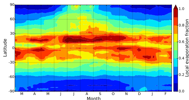
Figure 6. Column total, zonally averaged evaporation expressed as a fraction of local precipitation formation for March 2005 to February 2006. Values shown are smoothed by a 30-day running mean.
