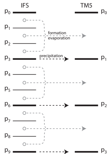
Figure 1. Regridding of additional meteorological fields in the coupling process between IFS and TM5. The mass flux of falling precipitation is directly sampled at the pressure levels shared by both modules. For precipitation formation and evaporation a volume-weighted average is calculated for multiple IFS pressure levels corresponding to one TM5 pressure level.
