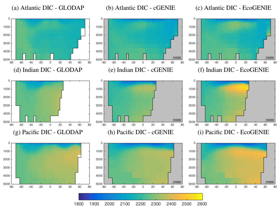
Figure 9. Basin-averaged meridional-depth distribution of DIC.
