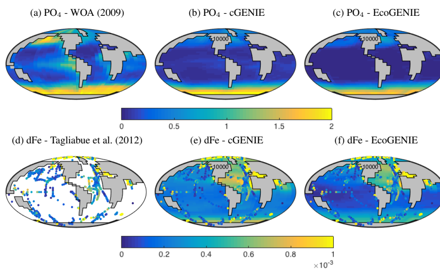
Figure 2. Surface concentrations of dissolved inorganic nutrients.
