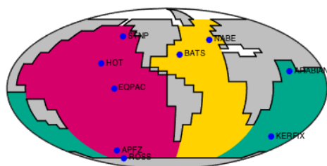
Figure 6. Spatial definition of the three ocean basins used in Figures 7 to 10. Locations of the JGOFS time-series sites are indicated with blue dots.
