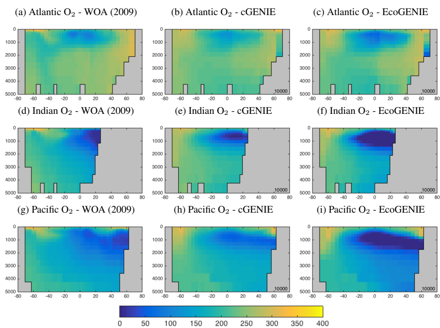
Figure 10. Basin-averaged meridional-depth distribution of dissolved oxygen.
