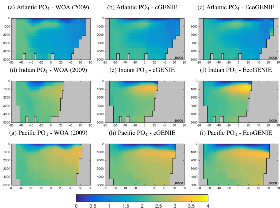
Figure 7. Basin-averaged meridional-depth distribution of phosphate.
