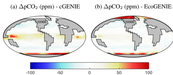
Figure 4. (Preindustrial) surface \Delta p\text{CO}_2 .
