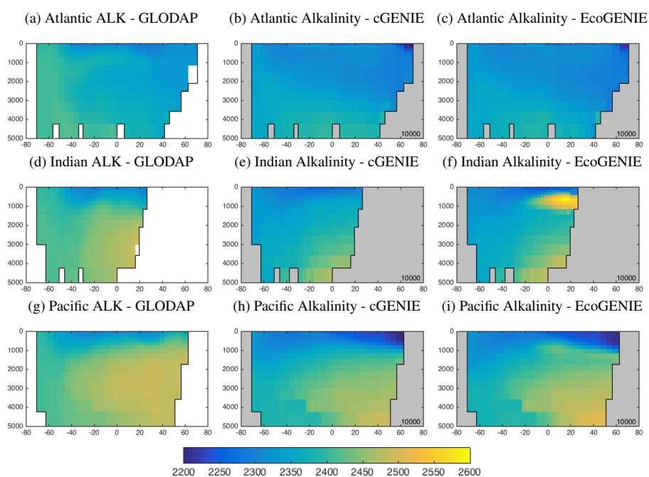
Figure 11. Basin-averaged meridional-depth distribution of alkalinity.
