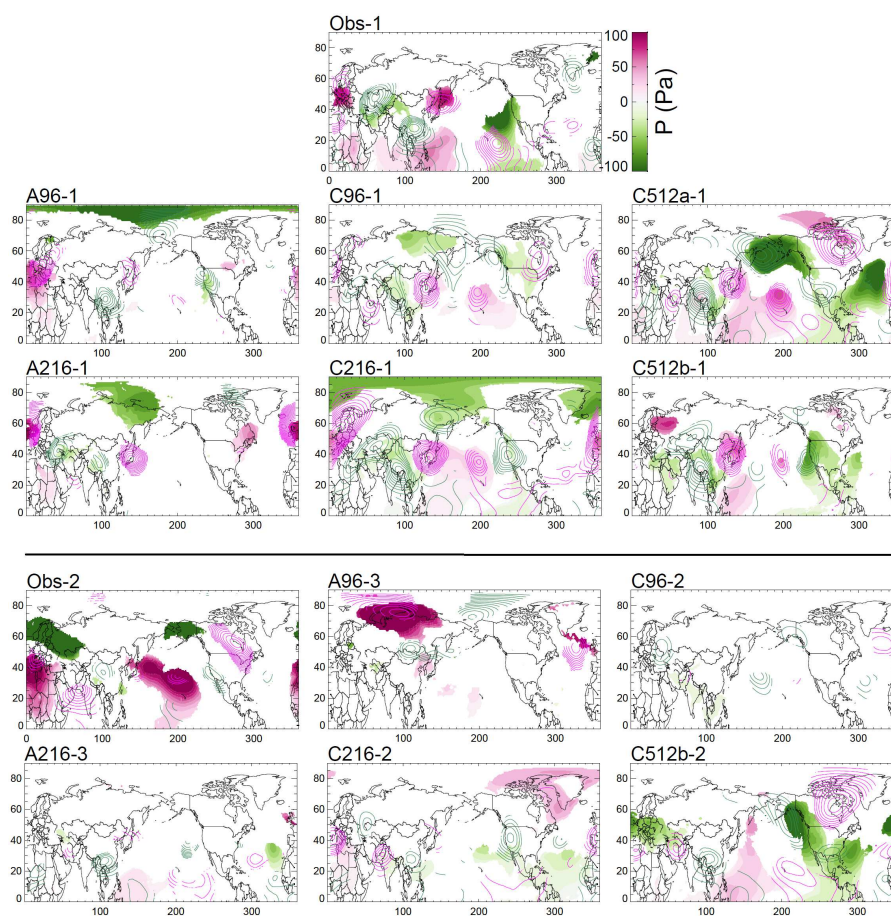
Figure 7. Regressions of P_{SFC} (shading) and Z_{200} (contours at intervals of 0.02 m, pink: positive, green: negative) against normalized DJF EOT timeseries. The top three (bottom two) rows are for EOTs matching the first (second) observed pattern. All shown values are significant at the 90 % confidence level.
