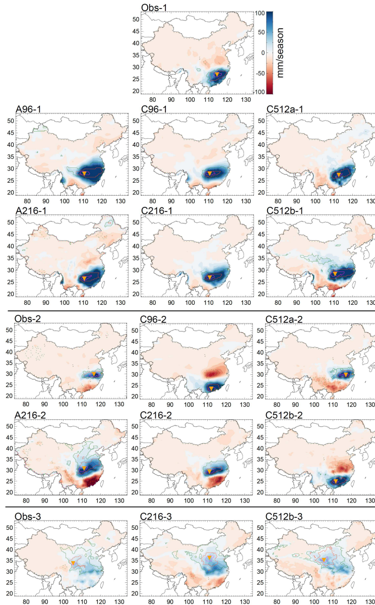
Figure 8. Shading shows regressions of MAM precipitation against observed or simulated EOT timeseries that have a linear correlation coefficient exceeding 0.38 with Obs-1 (top), Obs-2 (middle) or Obs-3 (bottom). Also shown are positive (solid lines) and negative (dashed lines) correlations of the full (leading order) or residual (higher order) precipitation-anomaly timeseries with the EOT base point exceeding 0.8 (magenta), 0.6 (orange), 0.4 (green). The EOT base point is marked by the orange inverted triangle. The number next to the simulation name above each panel indicates the order of the simulated EOT pattern.
