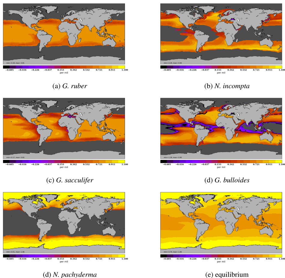
Figure 6. \delta^{18}\text{O}_e response to a horizontally and vertically homogeneous 4^\circ\text{C} cooling applied to the WOA13 dataset, \Delta^{18}\text{O}_e . Results are expressed in per mil for each species (panels (a-d)) and for the equilibrium surface calcite approach.
