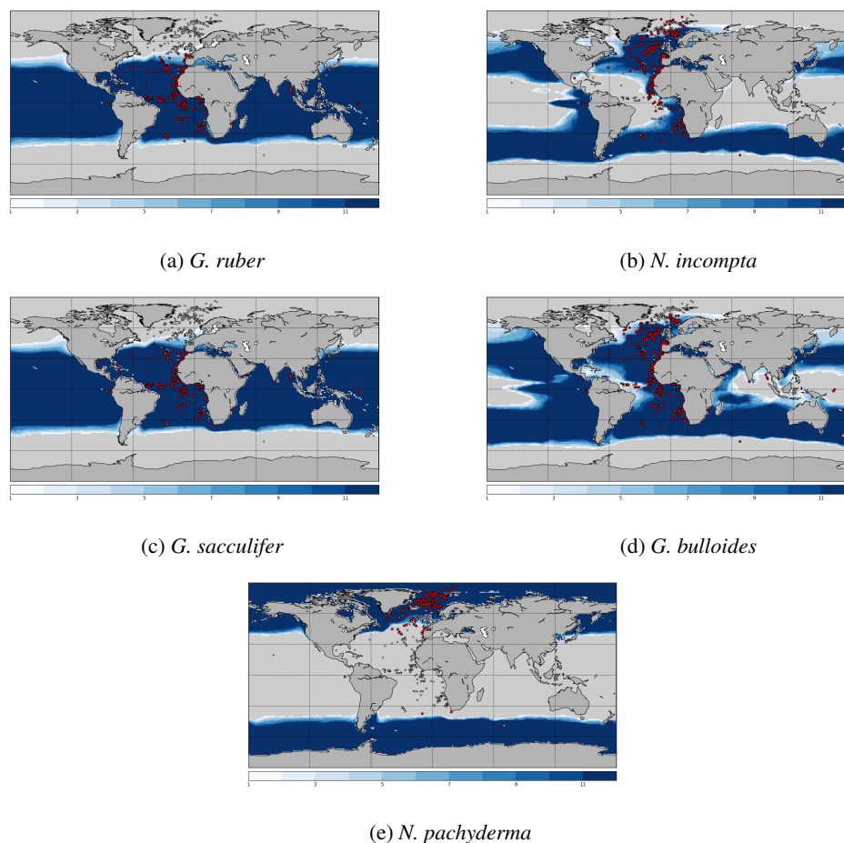
Figure 3. Model-data comparison of species abundances. Ocean regions where FAME predicts that the species is present at some time of the year ( \mu' > 0 ) are plotted in blue, with shades of blue indicating the number of months of presence. Overlaid are the MARGO Late Holocene data: sites where the species' abundance is higher than or equal to 10% are shown by red dots while the other sites are marked by white dots.
