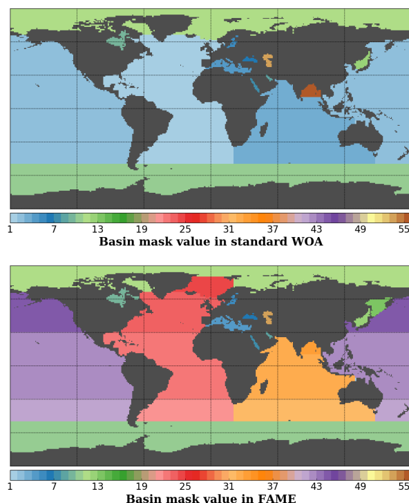
Figure A1. Basin masks as defined in the WOA standard mask file (above) and in FAME, on the same 1° resolution grid. Values corresponds to the basins defined in Table A1.
