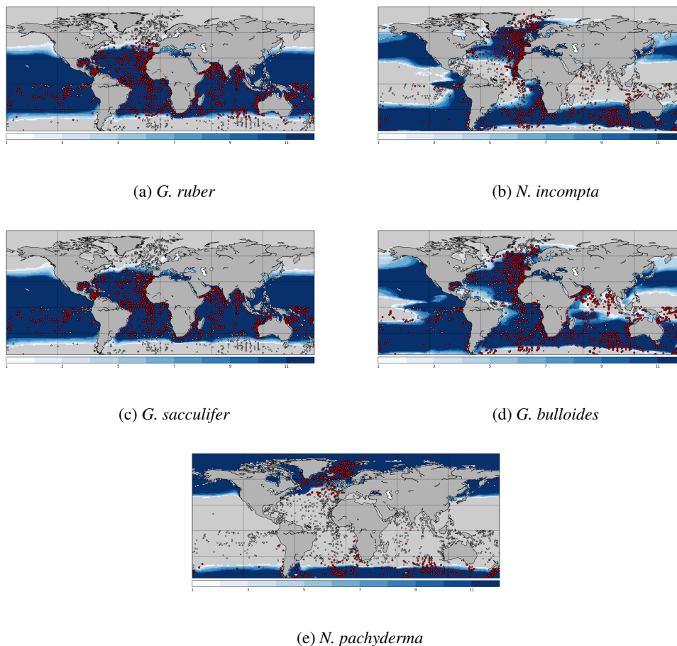
Figure A2. Model-data comparison of species abundances. Ocean regions where FAME predicts that the species is present at some time of the year ( \mu' > 0 ) are plotted in blue, with shades of blue indicating the number of months of presence. Overlaid are the MARGO Late Holocene data: sites where the species' abundance is higher than or equal to 10% are shown by red dots while the other sites are marked by white dots.
