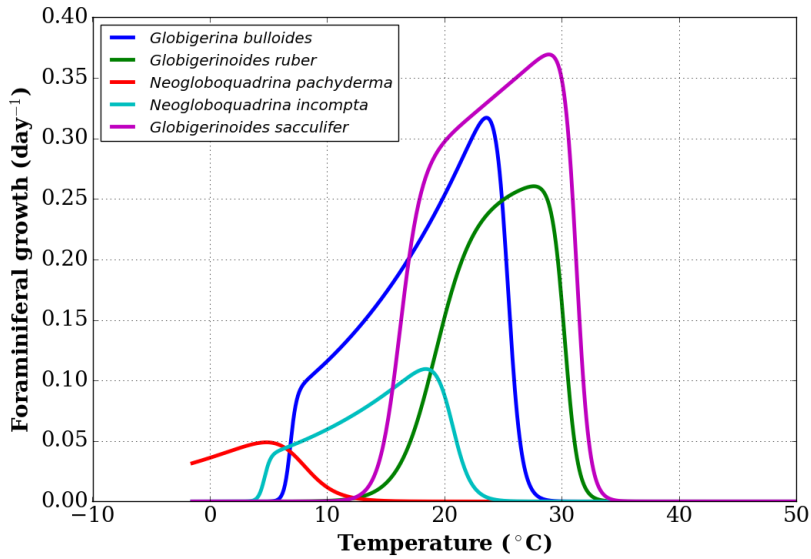
Figure 1. Growth functions corresponding to equation (1) over the full temperature range.
