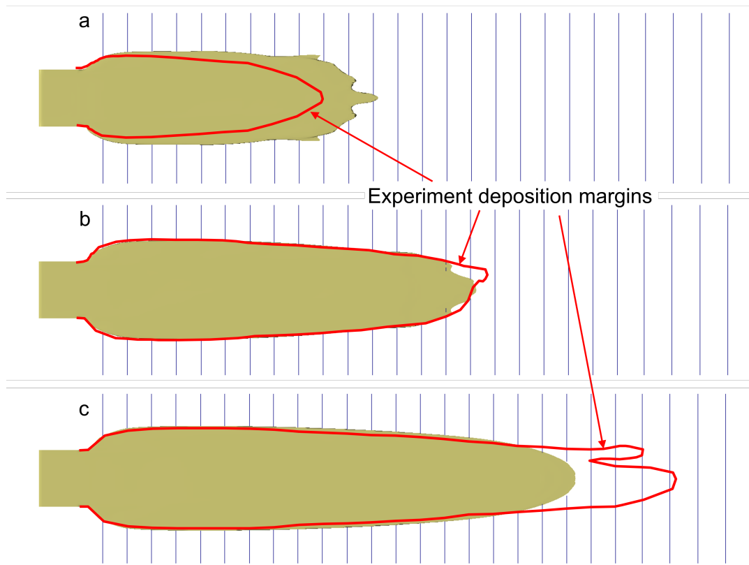
Figure 4. Simulated deposits (brown areas) and corresponding experiment deposition margins for mixtures with 27.0% (a), 28.5% (b) and 30% water content (c) applying \delta = 36^\circ and \tau_{00} based on the calibration case of 28.5% water content. The vertical thin lines represent the 20 cm spacing marks in the hillslope debris flow flume (Fig.1).
