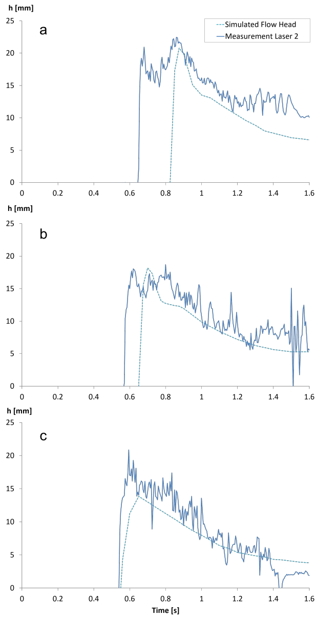
Figure 3. Laser measurement and corresponding simulated values of the flow depth over time, one meter down-slope of the gate for experiments with water contents of 27% (a), 28.5% (b) and 30% (c). The laser data were box-averaged over 10 milliseconds.
