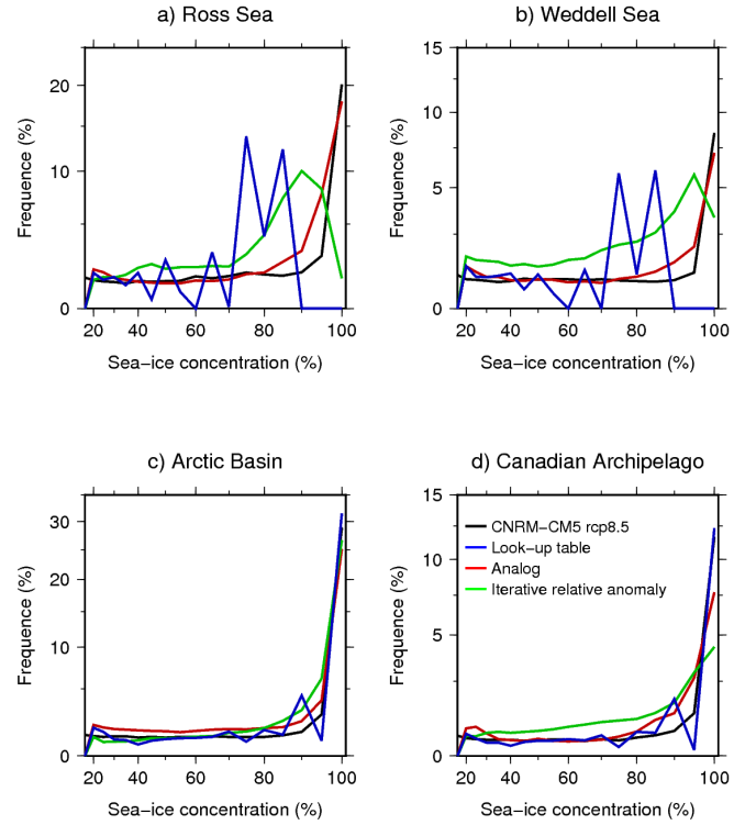
Figure 6. Frequency distribution of SIC in CNRM-CM5 RCP8.5 scenario (black) and in estimation using different methods in a perfect model test: Look-up table (blue), analog (red), and iterative relative anomaly (green). Regions are: a) Ross Sea ( 72^{\circ}\text{S};77^{\circ}\text{S}, 174^{\circ}\text{E};163^{\circ}\text{W} ); b) Weddell Sea ( 63^{\circ}\text{S};73^{\circ}\text{S}, 43^{\circ}\text{W};25^{\circ}\text{W} ); c) Arctic Basin ( 80^{\circ}\text{N};90^{\circ}\text{N}, 180^{\circ}\text{W};180^{\circ}\text{E} ); d) Canadian Archipelago ( 66^{\circ}\text{N};88^{\circ}\text{N}, 130^{\circ}\text{W};80^{\circ}\text{W} )
