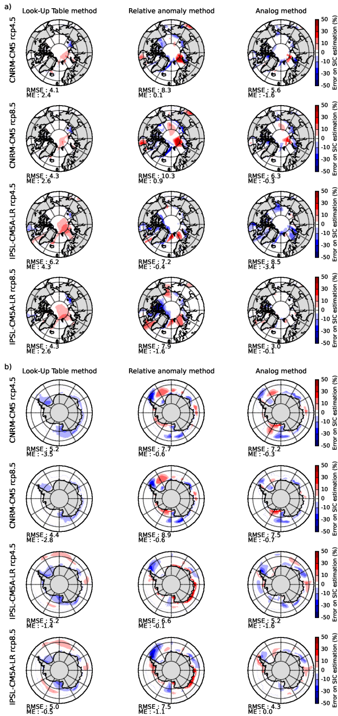
Figure 5. Mean error on the estimation of SIC with respect to the original AOGCM future scenario for the LUT, iterative relative anomaly and analog methods with CNRM-CM5 and IPSL-CM5A-LR RCP4.5 and RCP8.5 scenarios for the Arctic (a) and the Antarctic (b)
