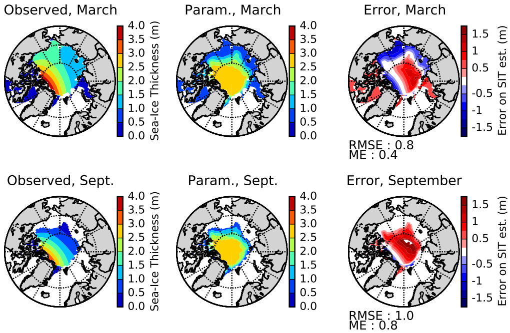
Figure 12. Observed (regressed, Lindsay and Schweiger (2015)) and parameterized Arctic SIT (in m) for March and September, and difference between these (right), with the global parameter set.
