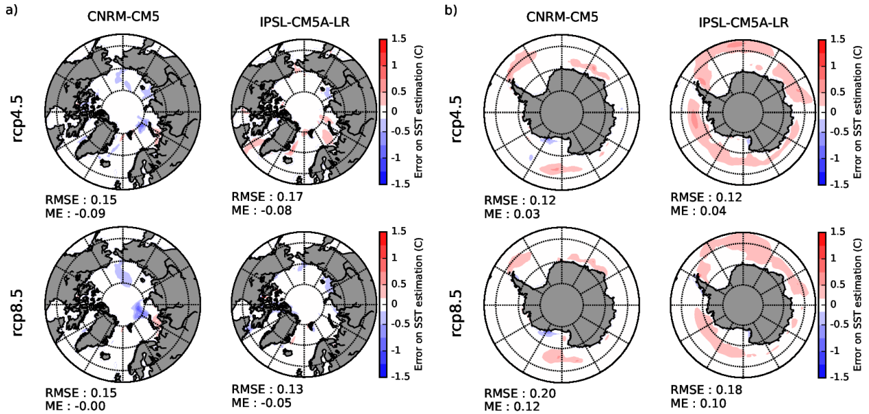
Figure 10. Mean error on the estimation of SST with respect to the corresponding original AOGCM scenario after applying the analog method for sea-ice, the quantile-quantile method for SST and the correction for SST and SIC consistency for the Arctic (a) and the Southern Oceans (b)
