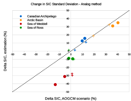
Figure 9. Change in bias-corrected SIC projections standard deviation using a) Look-Up Table, b) iterative relative anomaly, c) analog methods against corresponding mean change in the AOGCM scenario for the four test regions : Canadian Archipelago (blue), Arctic Basin (orange), Weddell Sea (red) and Ross Sea (green). Circles represent scenarios (rcp4.5 and rcp8.5) of CNRM-CM5 and crosses, scenarios of IPSL-CM5A-LR
