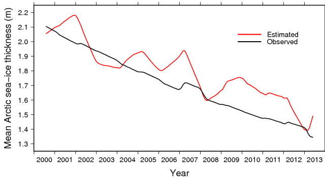
Figure 11. Observed (black, after (Lindsay and Schweiger, 2015)) and diagnosed (red) 12-month moving average mean sea-ice SIT of the Arctic basin (see Figure 12). The global parameter set is used here. Slight differences to Figure 13 of Lindsay and Schweiger (2015) appear because here we mask ice-free (SIC < 15%) areas that have a finite, non-zero ice thickness in the regression proposed by Lindsay and Schweiger (2015) who extend their regression to the entire Arctic Basin at all seasons.
