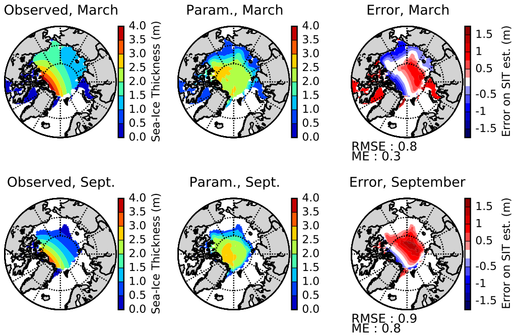
Figure 15. Observed Lindsay and Schweiger (2015) and parameterized Arctic SIT (in m) for March and September, and difference between these (right), with the Arctic-specific parameter set.
