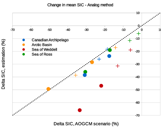
Figure 8. Change in mean bias-corrected SIC projections using a) Look-Up Table, b) iterative relative anomaly, c) analog methods against corresponding mean change in the AOGCM scenario for the four test regions : Canadian Archipelago (blue), Arctic Basin (orange), Weddell Sea (red) and Ross Sea (green). Circles represent scenarios (rcp4.5 and rcp8.5) of CNRM-CM5 and crosses, scenarios of IPSL-CM5A-LR
