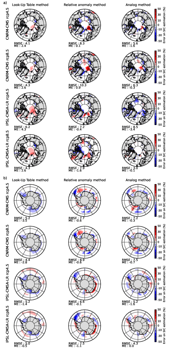
Figure 6. Mean error on the estimation of SIC with respect to the original AOGCM future scenario for the LUT, iterative relative anomaly and analog methods with CNRM-CM5 and IPSL-CM5A-LR rcp4.5 and rcp8.5 scenarios for the Arctic (a) and the Antarctic (b)
