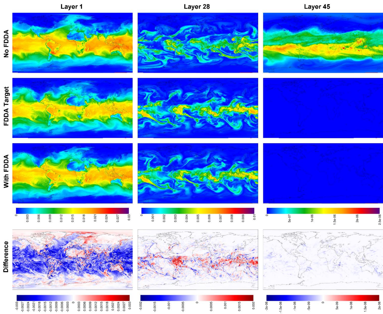
Figure 6: MPAS-A simulation results without FDDA (top row), FDDA target fields, MPAS-A results with FDDA, and FDDA target minus MPAS-A with FDDA (bottom row) for water vapor mixing ratio (kg kg -1 ) in layers 1, 28, and 45, for 00 UTC on 31 January 2013, 30 days into the simulation.
