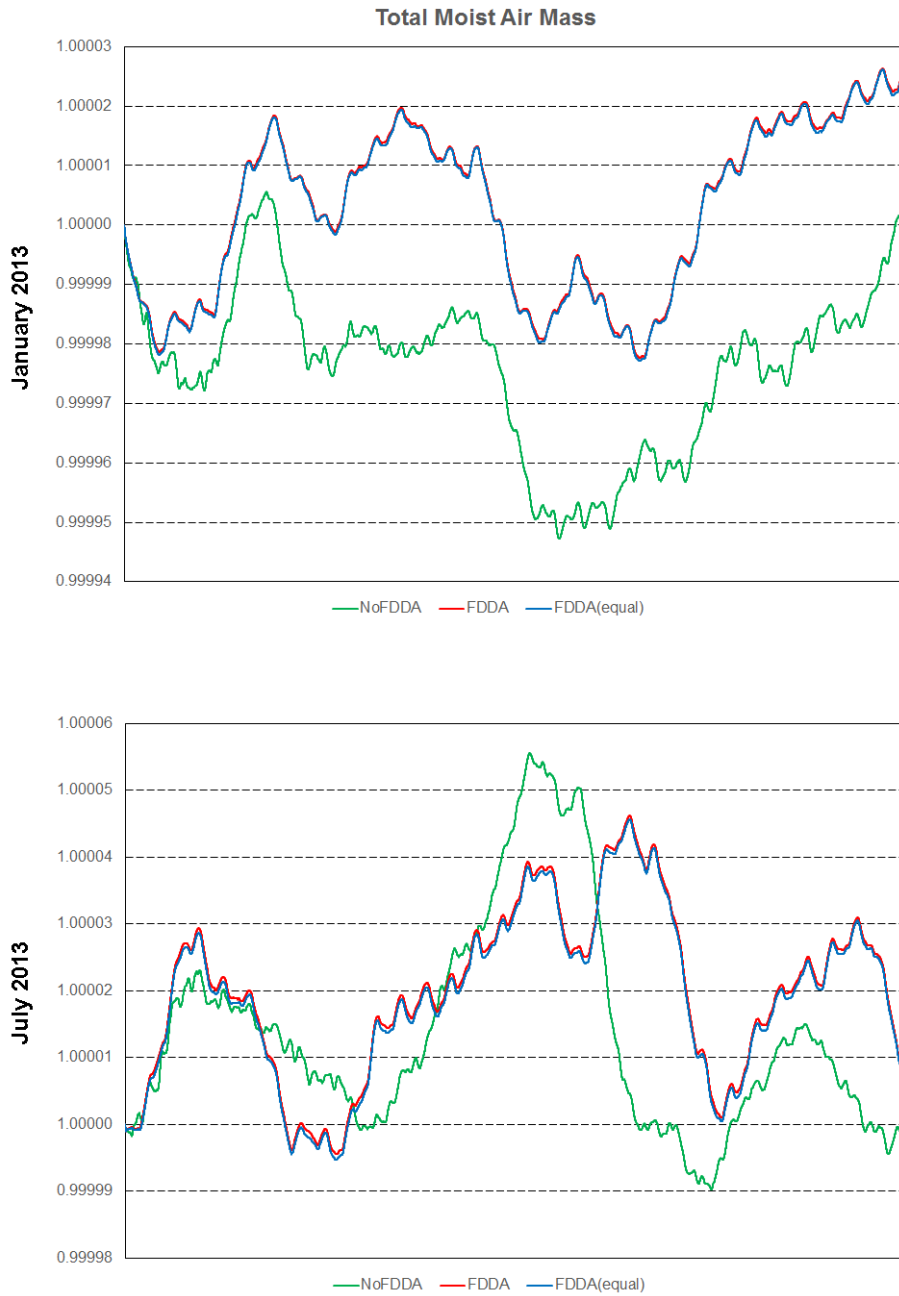
Figure 18: Time-series plots of total moist air mass (left column), total water vapor mass (center column), and total dry air mass (right column) scaled to their initial values for the two test periods. Results are from MPAS-A without FDDA (green line), MPAS-A using weaker q_v nudging (red line), and MPAS-A using equal nudging for all variables (blue line).
