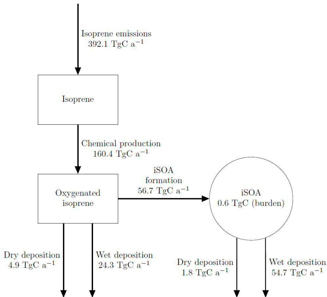
Figure 4. Global budgets for isoprene derived secondary organic aerosol and its precursors (sources/sinks in TgC a -1 and burden in TgC) predicted by ECHAM-HAMMOZ reference simulation for 2012. For details about the individual compounds see Table 3.
