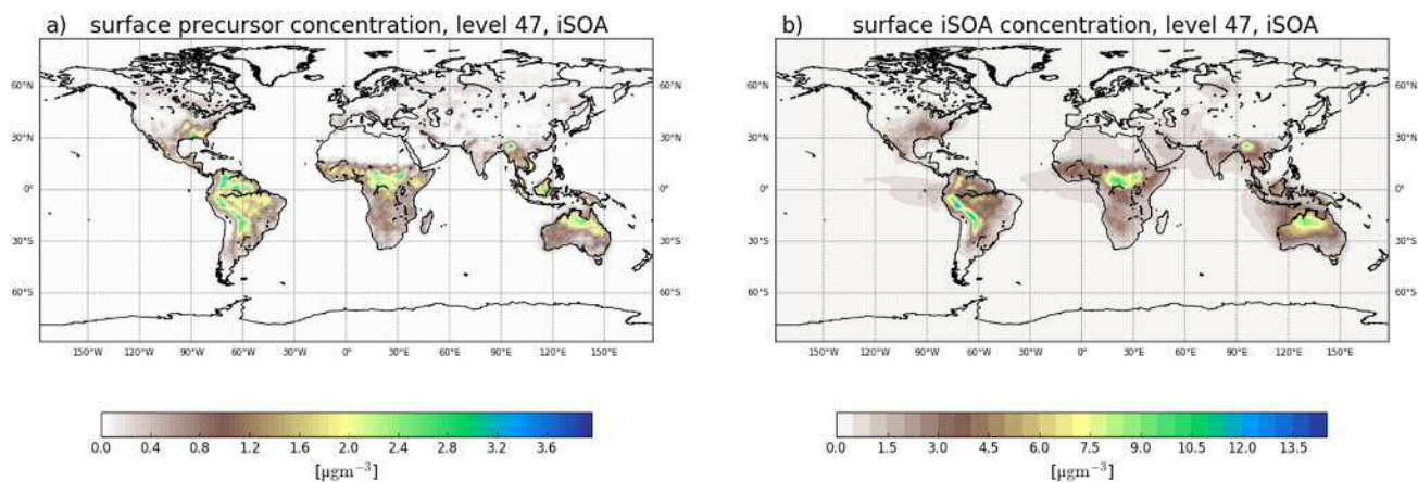
Figure 2. Global surface layer maps showing, the iSOA precursor gas phase concentration in plot a) and the aerosol phase iSOA concentration in plot b) as annual averages for 2012 in \mu\text{g m}^{-3} . The reader should note the different color scales, higher concentrations are reached in the aerosol phase, plot b).
