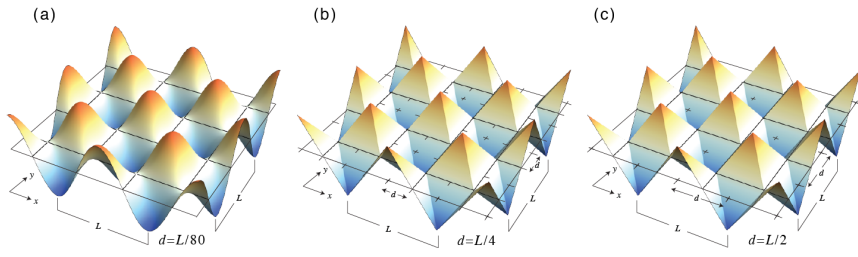
Figure 12: Initial perturbations used in the simulations with the Z, C, CD and D grid models for the grid spacings of (a) d = L/80 , (b) d = L/4 , and (c) d = L/2 .
