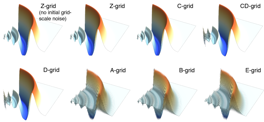
Figure 13: Horizontal structure of the inertia-gravity wave simulated by the various horizontal grids after 100 mins of integration.
