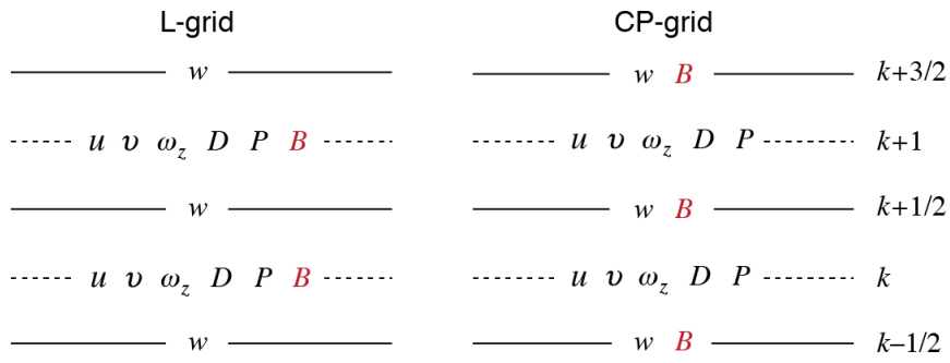
Figure 10: The L (left panel) and CP (right panel) grids and the distribution of variables.
