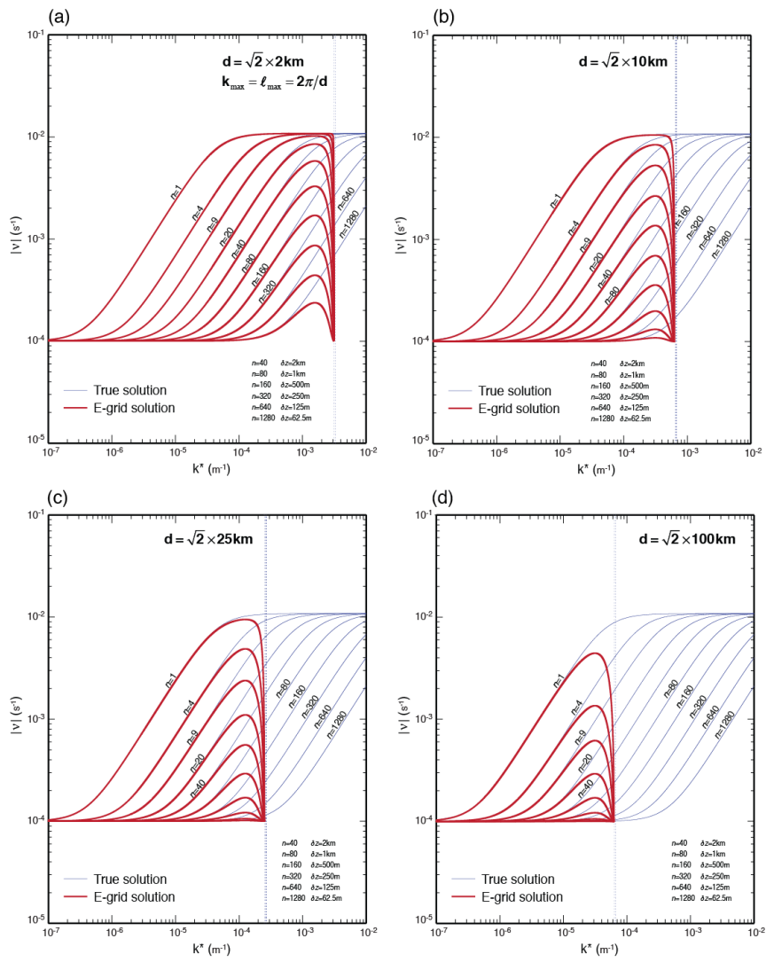
Figure 8: Same as Fig. 2, but for the E grid.
