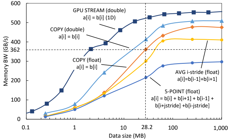
Figure A1. Bandwidth of the representative stencil benchmarks and GPU-STREAM on Tesla P100. All kernels (except of for GPU STREAM) operate on a 3D domain.
