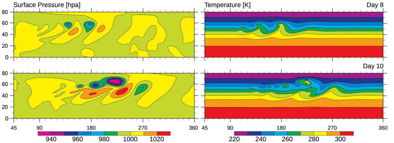
Figure 3. Evolution of the a baroclinic wave in a dry simulation with 47 km grid spacing on day 8 and 10: (Left) Surface Pressure and (right) temperature on the 850 hPa pressure level (roughly 1.5 km above sea level).
