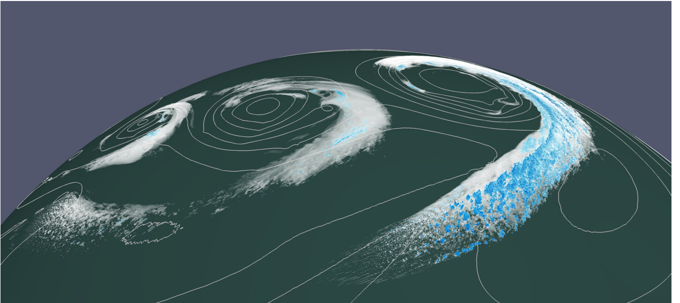
Figure 1. Visualization of the a baroclinic wave at day 10 of the a simulation with 930 m grid spacing. (White shading) Volume render of cloud ice, cloud water, and graupel \geq 10^{-3} g/kg. (Blue shading) Isosurface of rain and snow hydrometeros hydrometeors \geq 4 \cdot 10^{-2} g/kg. The white contours denote surface pressure.
