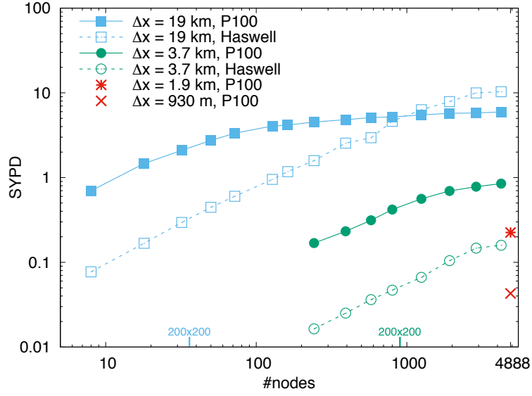
Figure 6. Strong scalability on Piz Daint: (Filled symbols) On : on P100 GPUs , and (empty-filled symbols), and on Haswell CPUs , using 12 MPI ranks per node (empty symbols).
