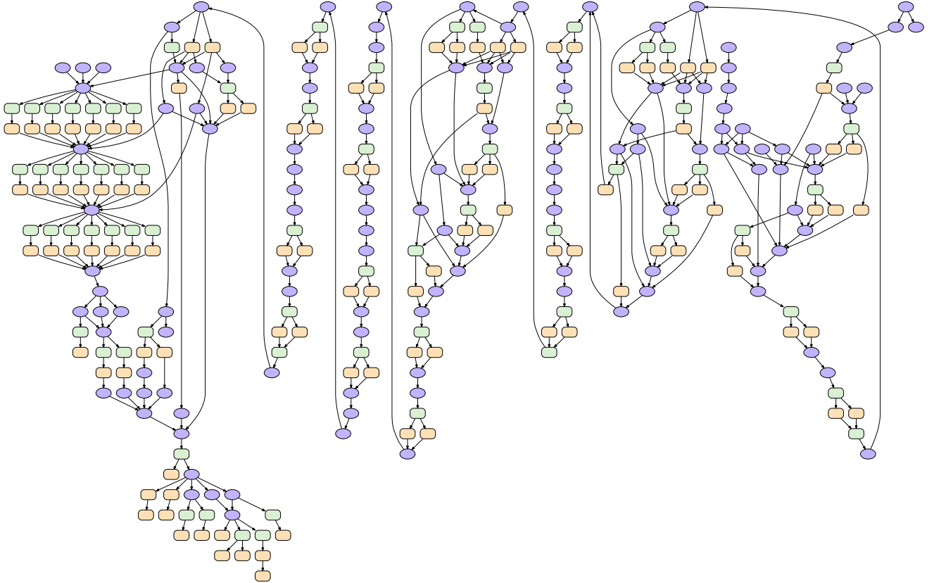
Figure 2. Illustration of the computational complexity of the COSMO dynamical core, using a Computational Directed Acyclic Graph (CDAG) of the COSMO dynamical core. The CDAG shows complex stencil operations nodes of the graph represent computational kernels (a kernel) that produce multiple fields (blue ellipses) as well as MPI that can have multiple input and output variables, halo exchanges (green rectangles) and boundary condition operations (orange rectangles). The edges of the graph represent data dependencies. Since the dynamical core of COSMO has been written using a domain-specific language (DSL), the CDAG can be produced automatically using an analysis backend of the DSL compiler. The lengthy serial section in the middle of the figure corresponds to the sound waves sub-stepping in the fast-waves solver. The parallel section on the upper-left corresponds to the advection of the seven tracer variables. CDAGs can automatically be produced from C++ code.
