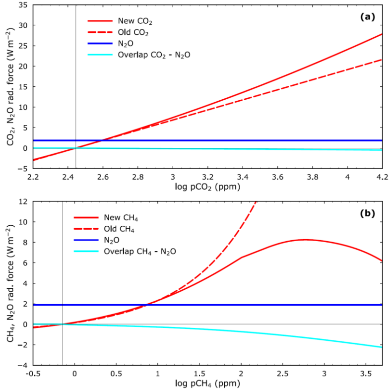
Figure 5: Radiative forcing of carbon dioxide, methane and nitrous oxide as functions of their atmospheric concentrations. a) CO 2 radiative forcing used here (new CO 2 ; Byrne and Goldblatt, 2014a) compared to CO 2 forcing in the original DCESS model (old CO 2 ; Shaffer et al., 2008). CO 2 -N 2 O overlap (Byrne and Goldblatt, 2014a) and N 2 O radiative forcing calculated for constant, pre-industrial N 2 O partial pressure of 270 ppb., b) CH 4 radiative forcing used here (new CH 4 ; Byrne and Goldblatt, 2014a,b) compared to CH 4 forcing in the original DCESS model (old CH 4 ). CH 4 -N 2 O overlap (Byrne and Goldblatt, 2014a) and N 2 O radiative forcing calculated for constant N 2 O partial pressure as in a .
