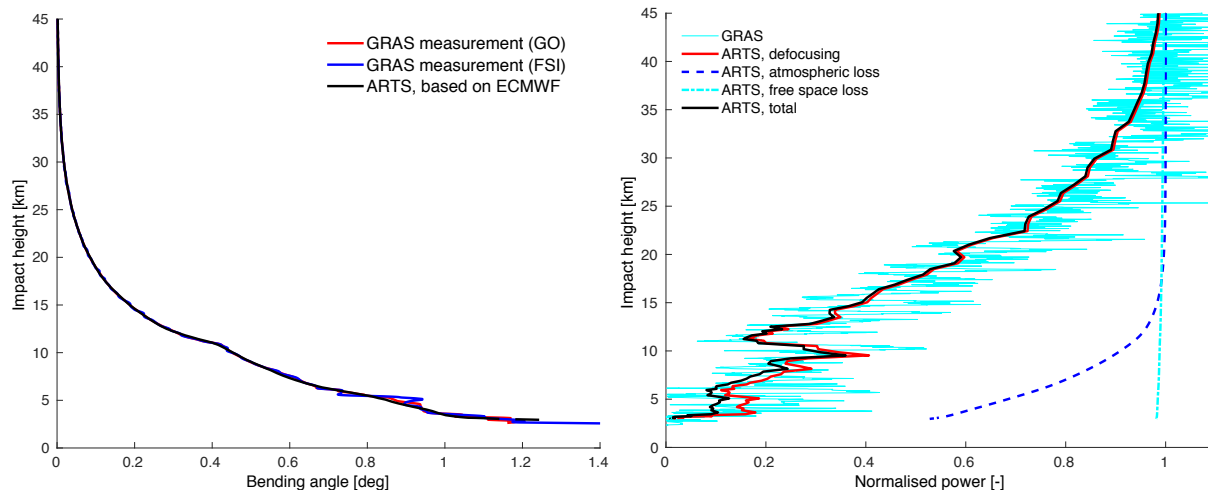
Figure 5. Comparison of ARTS forward model calculations with GRAS data. The input to ARTS is ECMWF operational analysis data. The left panel compares ARTS simulations to observed bending angles determined in two different ways from raw GRAS observations. The right panel shows the observed and simulated link budget for transmitted power. As common for radio-occultation observations, the vertical scale, impact height, is simply the impact parameter of Figure 4 minus the Earth radius.
