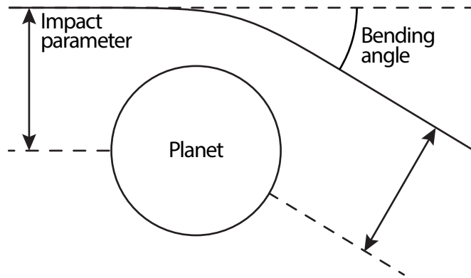
Figure 4. The radio occultation geometry with impact parameter and bending angle. See for example Kursinski et al. (2000) for details.
