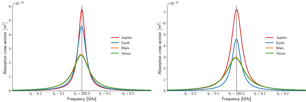
Figure 2. Absorption cross section of the 183 GHz water vapor line at 700 Pa, for the different atmospheric compositions listed in Table 2, assuming a Voigt line shape function. Left: using the Earth atmosphere temperature for all four cases, so that differences are only due to the different pressure broadening coefficients. Right: Taking also the temperature from the different planet scenarios, which affects the line strength, corresponding to the integral under the curves.
