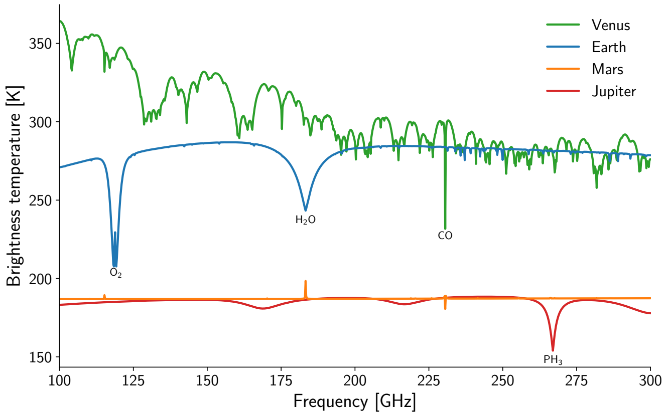
Figure 1. Simulated millimeter-wave nadir observations from space for four different planets. The atmospheric scenarios are the same as the ones behind Table 2 (vertical profiles, although the table just lists the data for a single pressure level). Surface reflectivity was assumed to be 0.4 for Earth, 0.13 for Mars, and does not play a role for the other two planets. The large spectral variability for Venus is caused by \text{SO}_2 .
