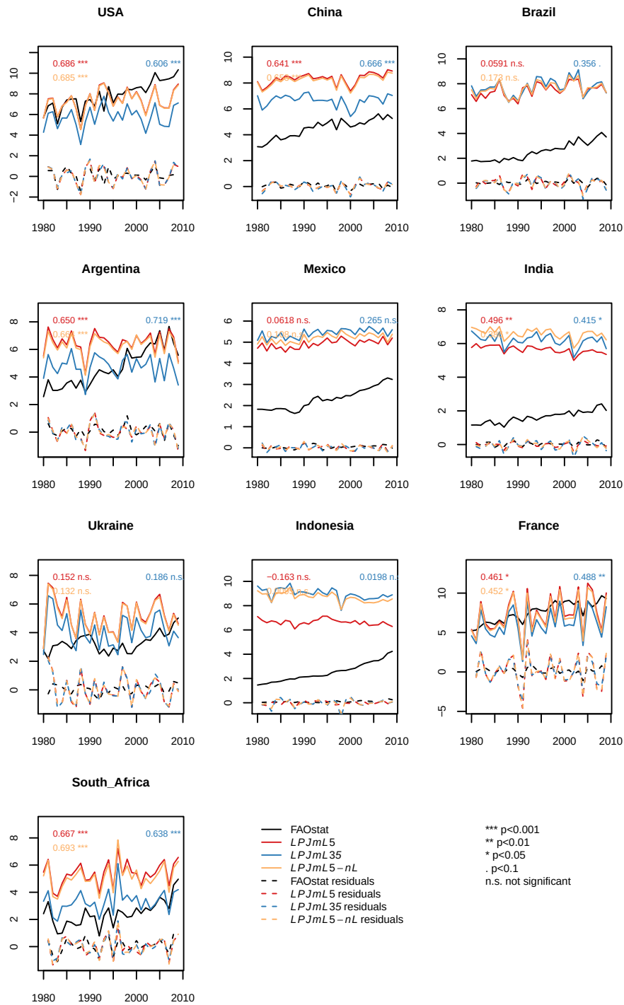
Figure 10. Maize yield simulations (in t fresh matter (FM) ha -1 ) for the 10 top-producing countries for the carbon-only LPJmL3.5 version (LPJmL35), the version with N limitation (LPJmL5) and with unlimited N supply (LPJmL5-nL). The residuals plotted are the detrended observed and simulated yields.
