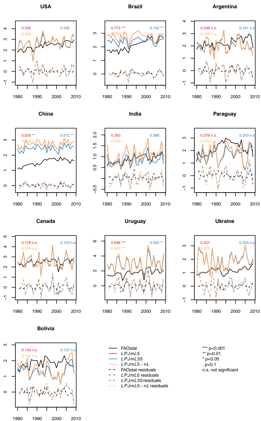
Figure S23. Soybean yield simulations (in tFM ha -1 ) for the 10 top-producing countries for the carbon-only LPJmL 3.5 version, the version with N limitation and with unlimited N supply.
