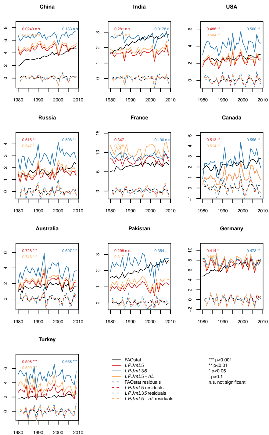
Figure S21. Wheat yield simulations (in \text{tFM ha}^{-1} ) for the 10 top-producing countries for the carbon-only LPJmL 3.5 version, the version with N limitation and with unlimited N supply.
