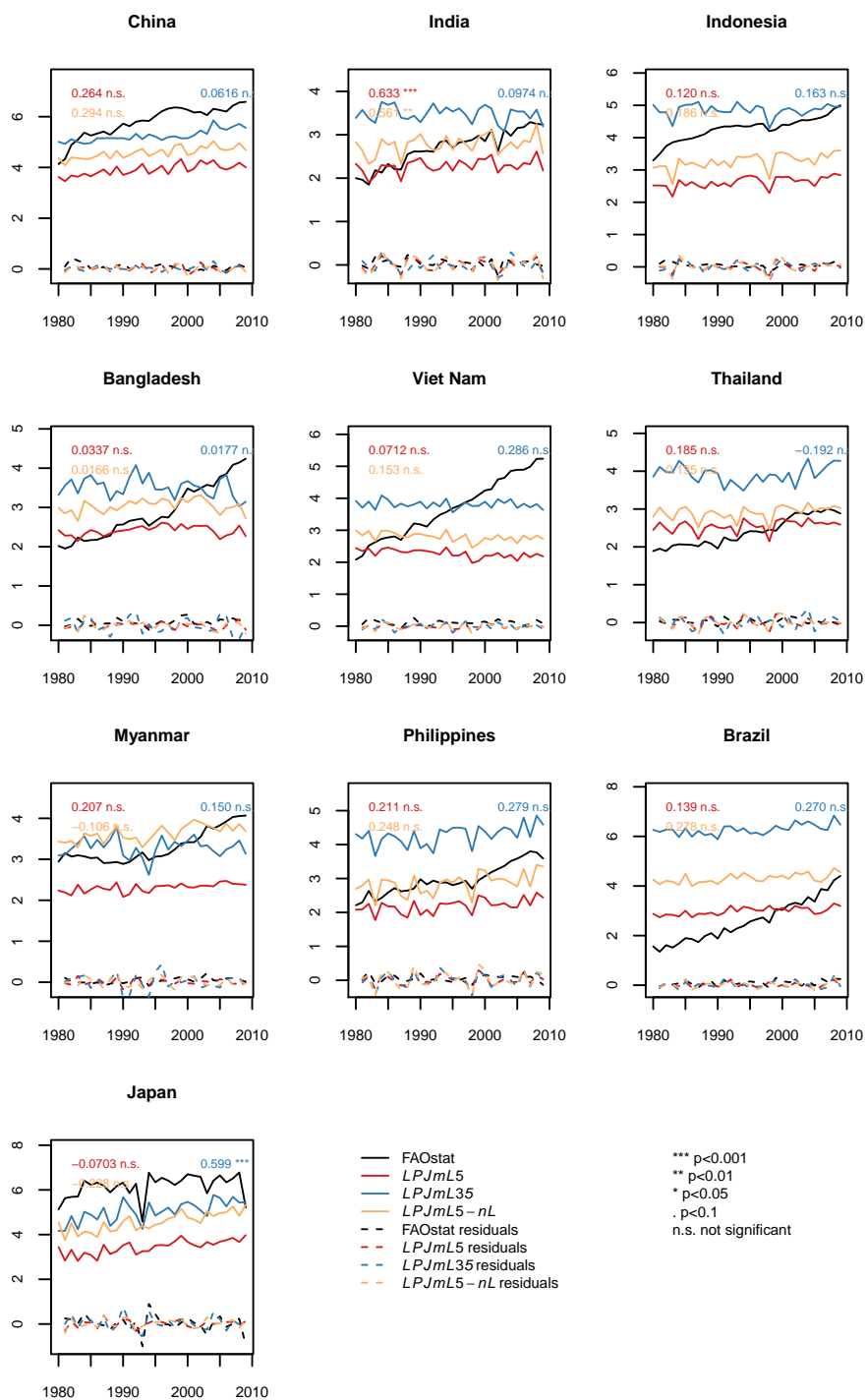
Figure S22. Rice yield simulations (in tFM ha -1 ) for the 10 top-producing countries for the carbon-only LPJmL 3.5 version, the version with N limitation and with unlimited N supply.
