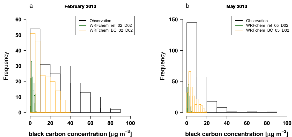
Figure 13. Black carbon concentrations at the Bode site, measured and simulated with WRF-Chem for February 2013 WRFchem_ref_02/05_D02 (a) and for May 2013 WRFchem_ref_02/05_D02 (b) as a histogram calculated from the 3-hourly values.
