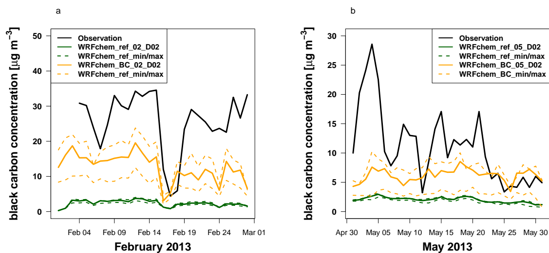
Figure 12. Time series of daily mean measured and simulated (WRFchem_ref_02/05_D02, WRFchem_BC_02/05_D02) black carbon concentrations [ \mu\text{g m}^{-3} ] at the Bode station for February (a) and May 2013 (b).
