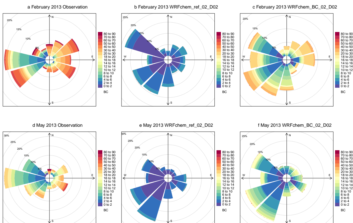
Figure 14. Pollution rose for black carbon at the Bode site calculated from the measured and simulated (WRFchem_ref_02/05_D02 and WRFchem_BC_02/05_D02) 3-hourly values of black carbon, wind speed and direction in February (a, b, c) and May (d, e, f) 2013. The figures represents the black carbon concentrations which coincide with a certain wind direction at the station and the frequency of occurrence of the wind direction in percent.
