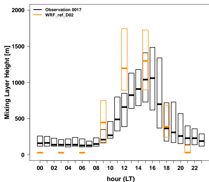
Figure 9. Diurnal cycle of the mixing layer heights [m] as a box-plot (showing the median, the upper and lower quantile) as diagnosed by the WRF model (WRF_ref_D02) and as determined from ceilometer measurement data at the Bode site for the period January - June 2013.
