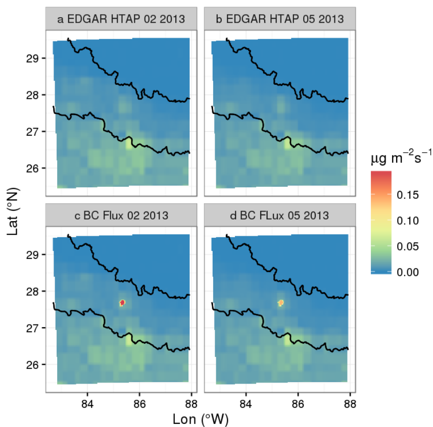
Figure 11. Black carbon emission flux used for the WRFchem_ref_02/05_D02 (a, b) and WRFchem_BC_02/05_D02 (c, d) simulations for February (left) and May 2013 (right) in \mu\text{g m}^{-2} \text{s}^{-1} .
