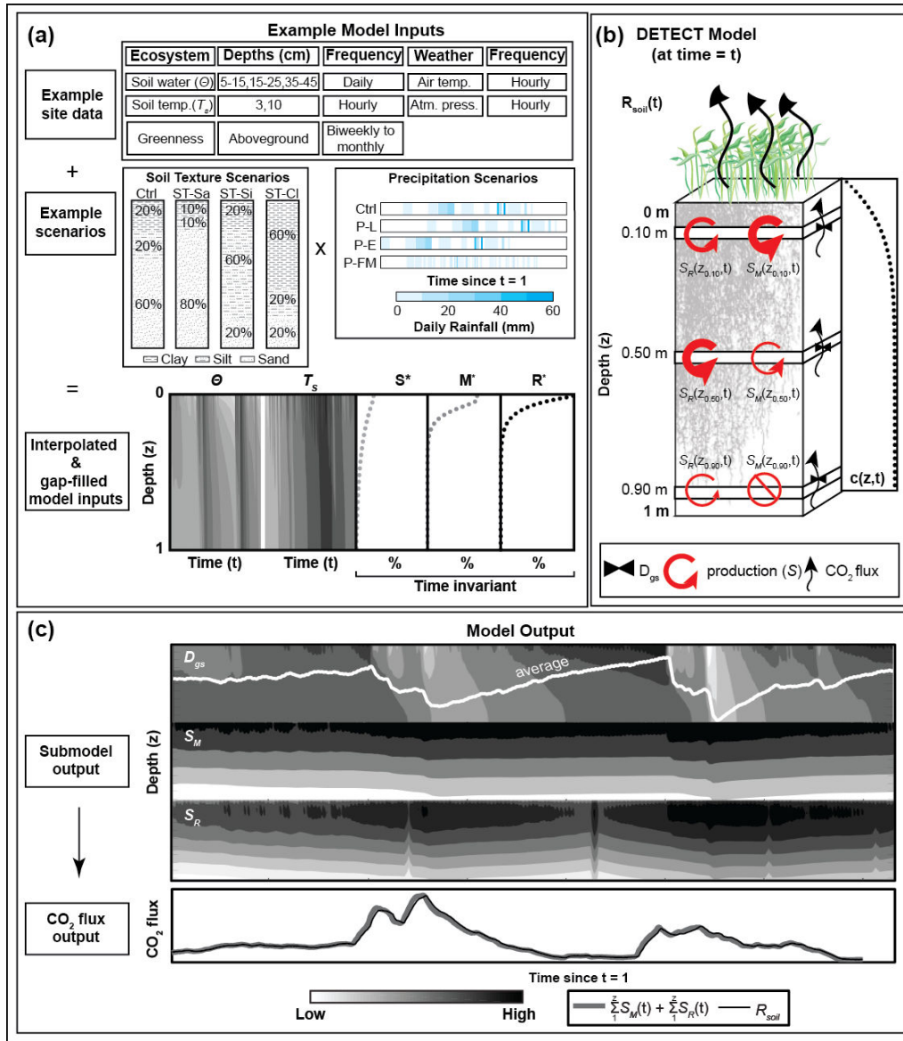
3 Figure 1. Graphical representation of (A) the required inputs to the DETECT model and the 4 associated scenarios implemented in this study, (B) the components of the DETECT model at a 5 particular time t , indicating depth-dependent production, \text{CO}_2 concentrations, and \text{CO}_2 fluxes, 6 and (C) example model outputs, such as temporally and spatially varying \text{CO}_2 diffusivity and 7 \text{CO}_2 production, and temporally varying bulk \text{CO}_2 fluxes.
