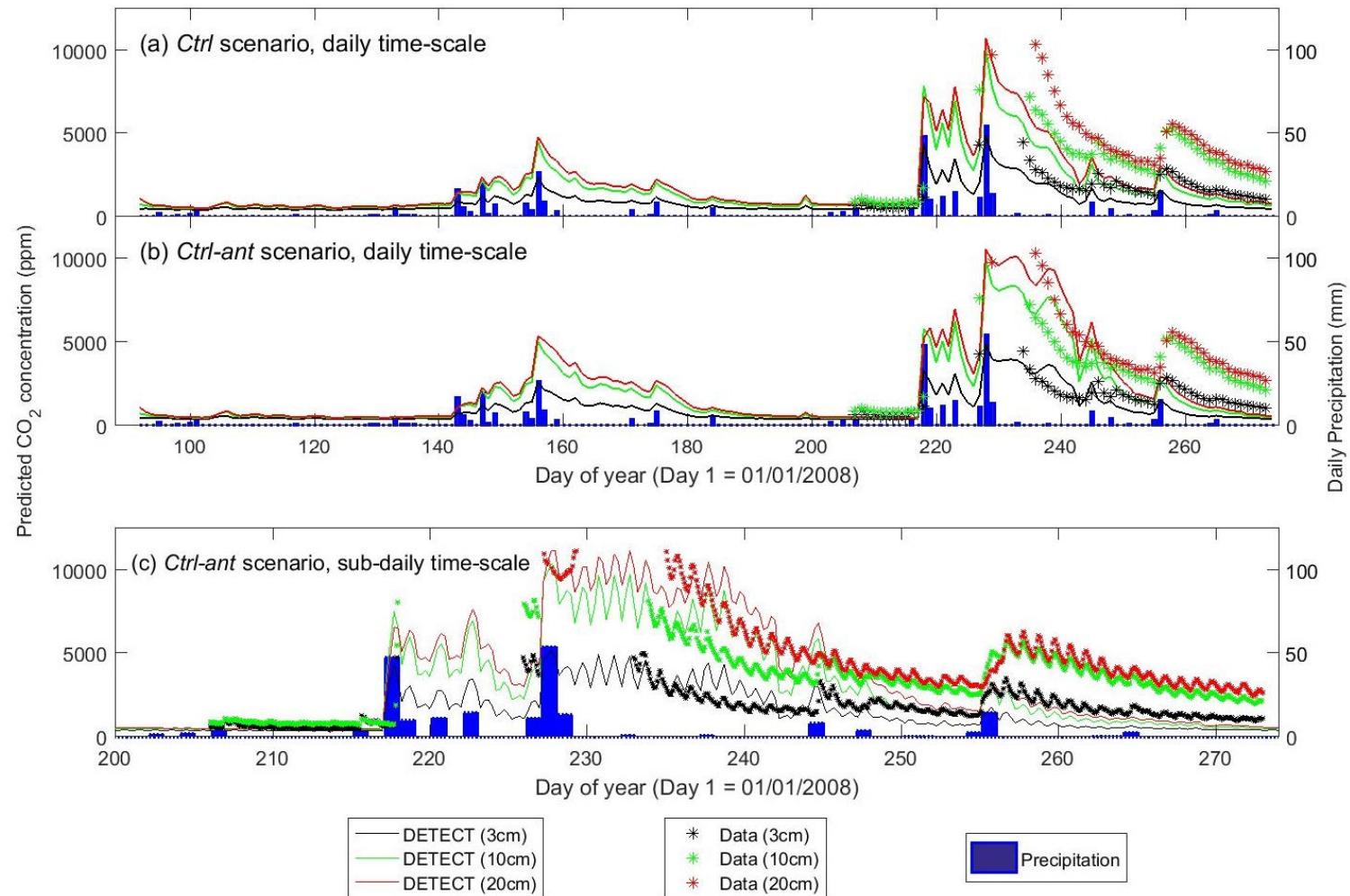
Figure 5 Time-series of predicted versus observed soil CO 2 concentrations at 3 cm depth, 10 cm depth, and 20 cm depth, where the predictions are based on the non-steady-state (NSS) DETECT model. Predicted [CO 2 ] is shown for the daily time-scale for the control scenarios (a) without ( Ctrl ) and (b) with ( Ctrl-ant ) antecedent effects, and for (c) the subdaily (every 6 hours) time scale for the Ctrl-ant scenario. Units are in parts per million (ppm).
