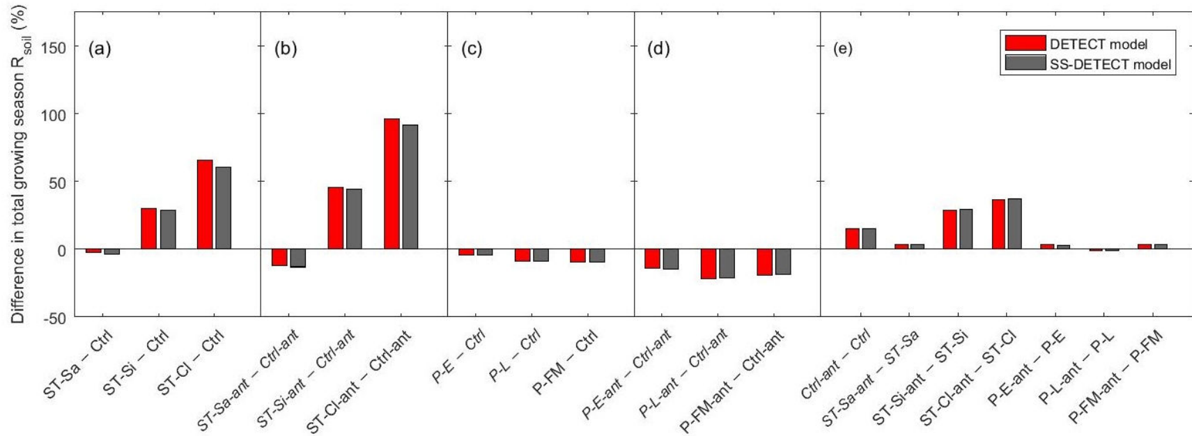
Figure 4 Differences of total growing season (April-September) soil respiration ( R_{soil} ) as predicted by the non-steady-state (DETECT) and steady-state (SS-DETECT) models, for different pairs of scenarios. Comparisons are grouped such that they quantify the effects of (a) soil texture without antecedent effects, (b) soil texture with antecedent effects, (c) precipitation without antecedent effects, (d) precipitation with antecedent effects, and (e) antecedent effects. See Table 2 for descriptions of each scenario .
