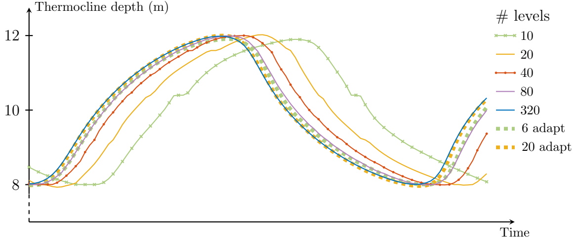
Figure 10. Convergence analysis for the internal seiche modelling. The graph shows the third oscillation of the seiche, at which moment the results are beginning to diverge from the high-resolution solution.
