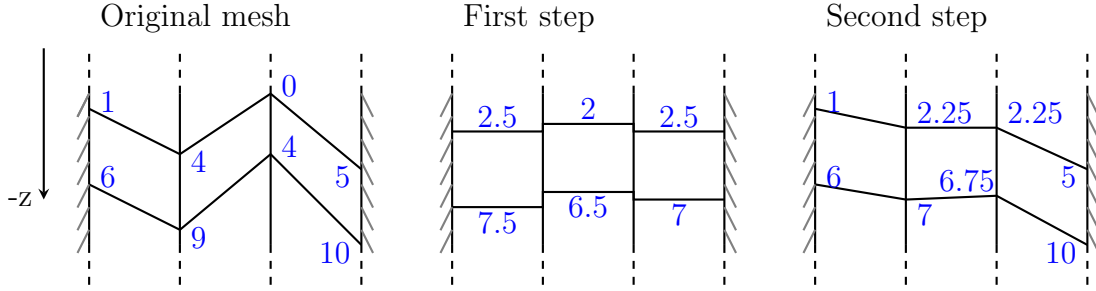
Figure 5. Illustration of the horizontal smoothing algorithm on a 2D “ x - z ” mesh. First, for each element, the upper and lower nodal values of the vertical coordinate z are set to their mean value, then z is projected onto a continuous field. The numbers refer to the depth of the mesh levels.
