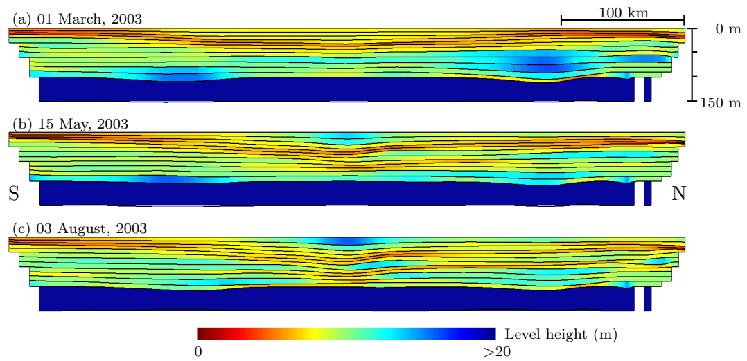
Figure 19. South-north level height thickness distribution transect on March 1st (a), May 15th (b) and August 3rd (c), 2003. Only the 150 upper metres vertical profile are displayed on the figure. The colormap is cropped at 20 m.
