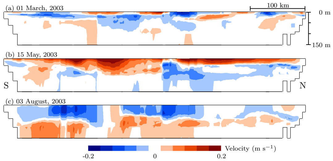
Figure 18. South-north velocity transect on March 1st (a), May 15th (b) and August 3rd (c), 2003. Only the 150 upper metres vertical profile are displayed on the figure. Positive value means northward current.
