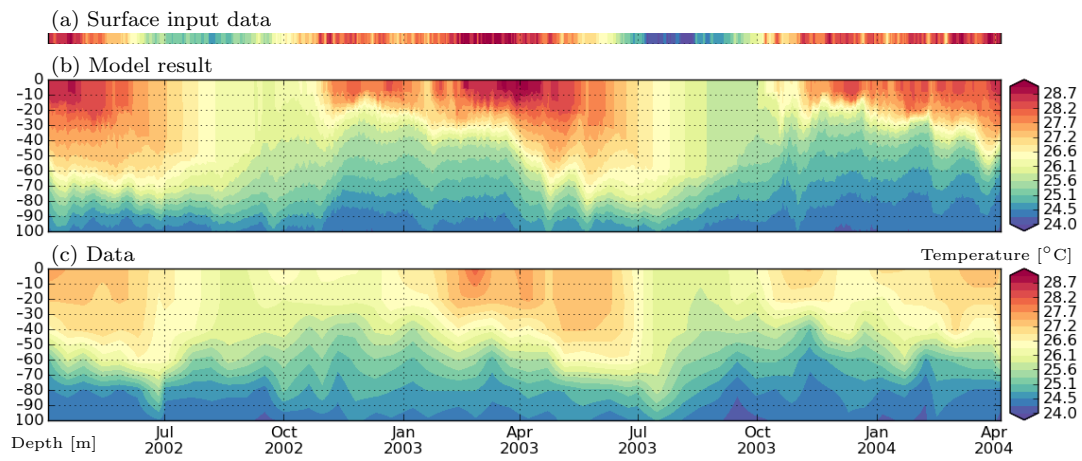
Figure 16. Lake water temperature (°C) at Kigoma as predicted by the model (b) and from in situ observations (c, Descy et al., 2006). Panel (a) shows the surface temperature used to force the temperature flux at the lake surface (Thiery et al., 2015).
