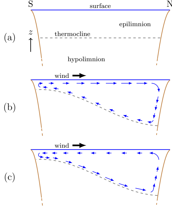
Figure 2. Schematical lake configuration with no wind stress (a) and with the south-easterly wind during the dry season in line with the classical circulation (b, Mortimer, 1961) such that the surface water follows the wind, or according to the non-classical circulation (c, Verburg et al., 2008) with reversed currents.
