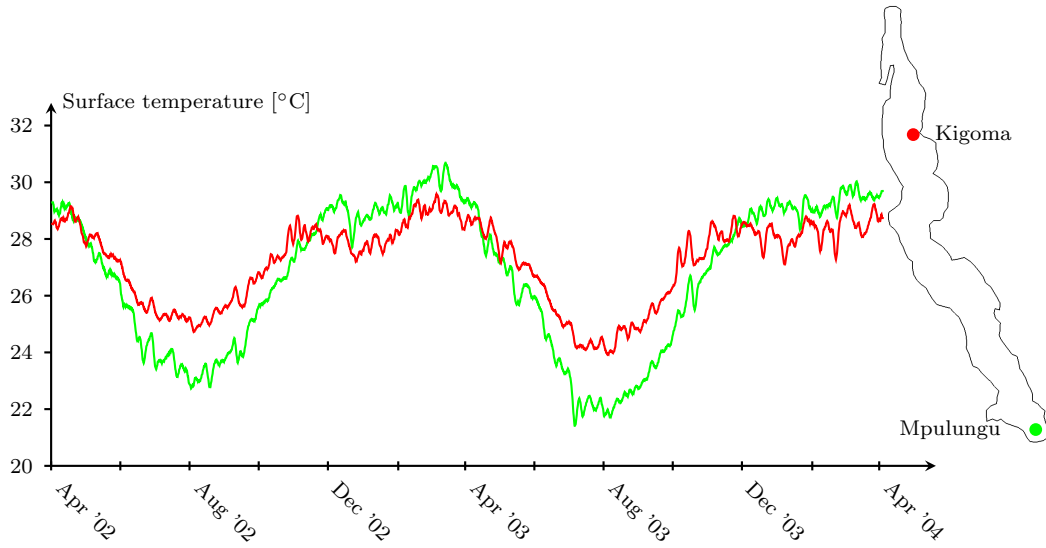
Figure 8. Time series of the surface temperature at Kigoma (red curve) and Mpulungu (green curve), as modelled by COSMO-CLM 2 (Thierry et al., 2015).
