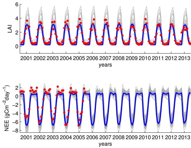
Figure 10. DALECV2 monthly estimates for LAI and NEE at Morgan Monroe State forest. The red dots are the observations, the blue trajectories are obtained using the 4DVAR analysis, the grey trajectories are ensemble runs obtained from a 95% confidence sample of the posterior pdf.
