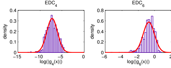
Figure 3. distribution and Gaussian fit for \text{EDC}_4 and \text{EDC}_6 .
