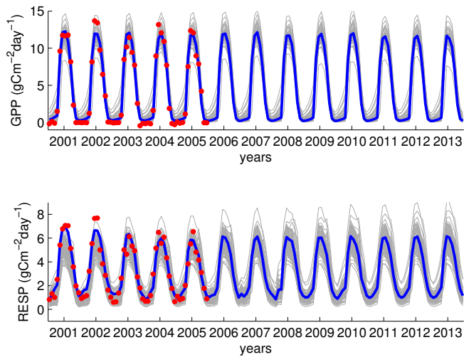
Figure 11. DALECV2 monthly estimates for GPP and RESP at Morgan Monroe State forest. The red dots are the observations, the blue trajectories are obtained using the 4DVAR analysis, the grey trajectories are ensemble runs obtained from a 95% confidence sample of the posterior pdf.
